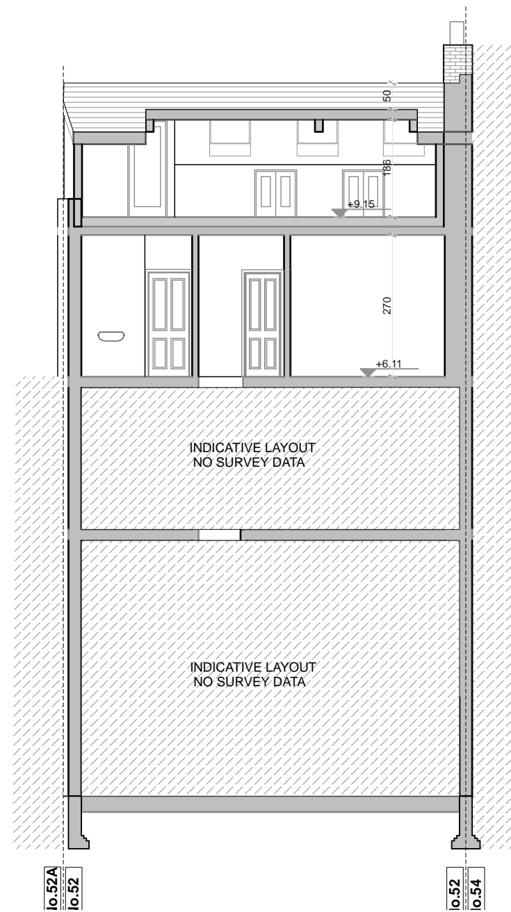
SECTION B-B PROPOSED
