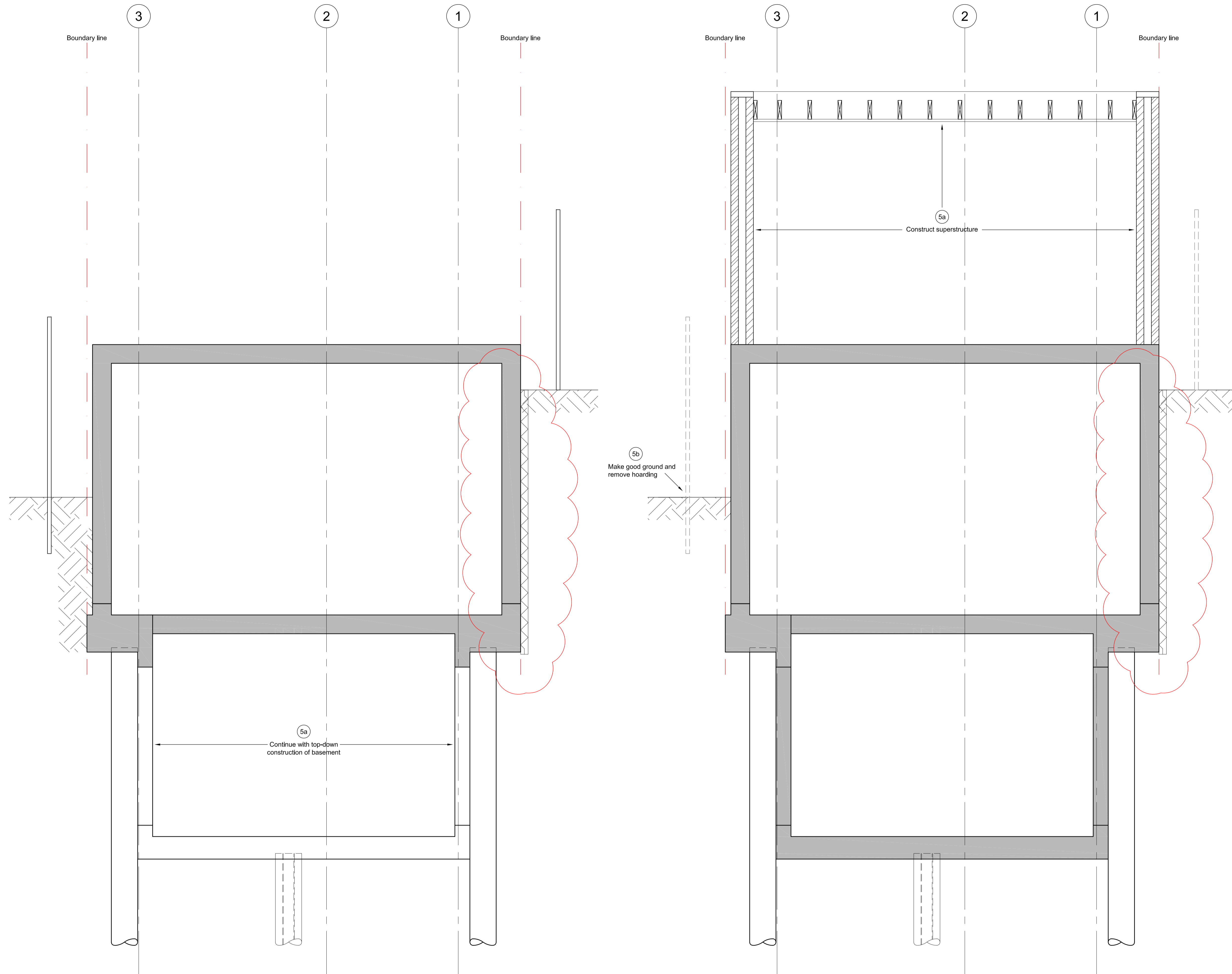
Stage 5 Scale 1:25
