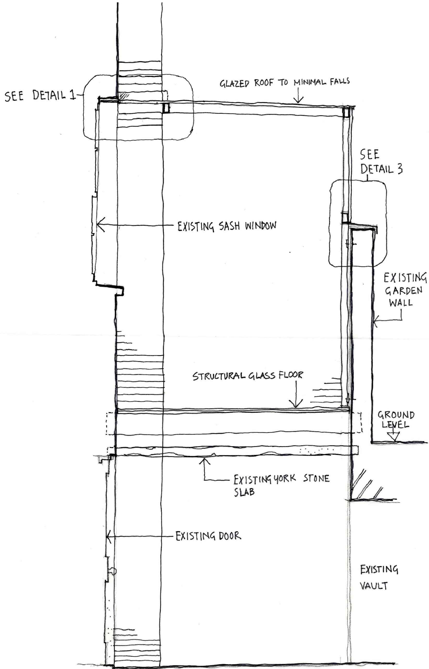
01 PROPOSED SECTION C-C scale 1:20
