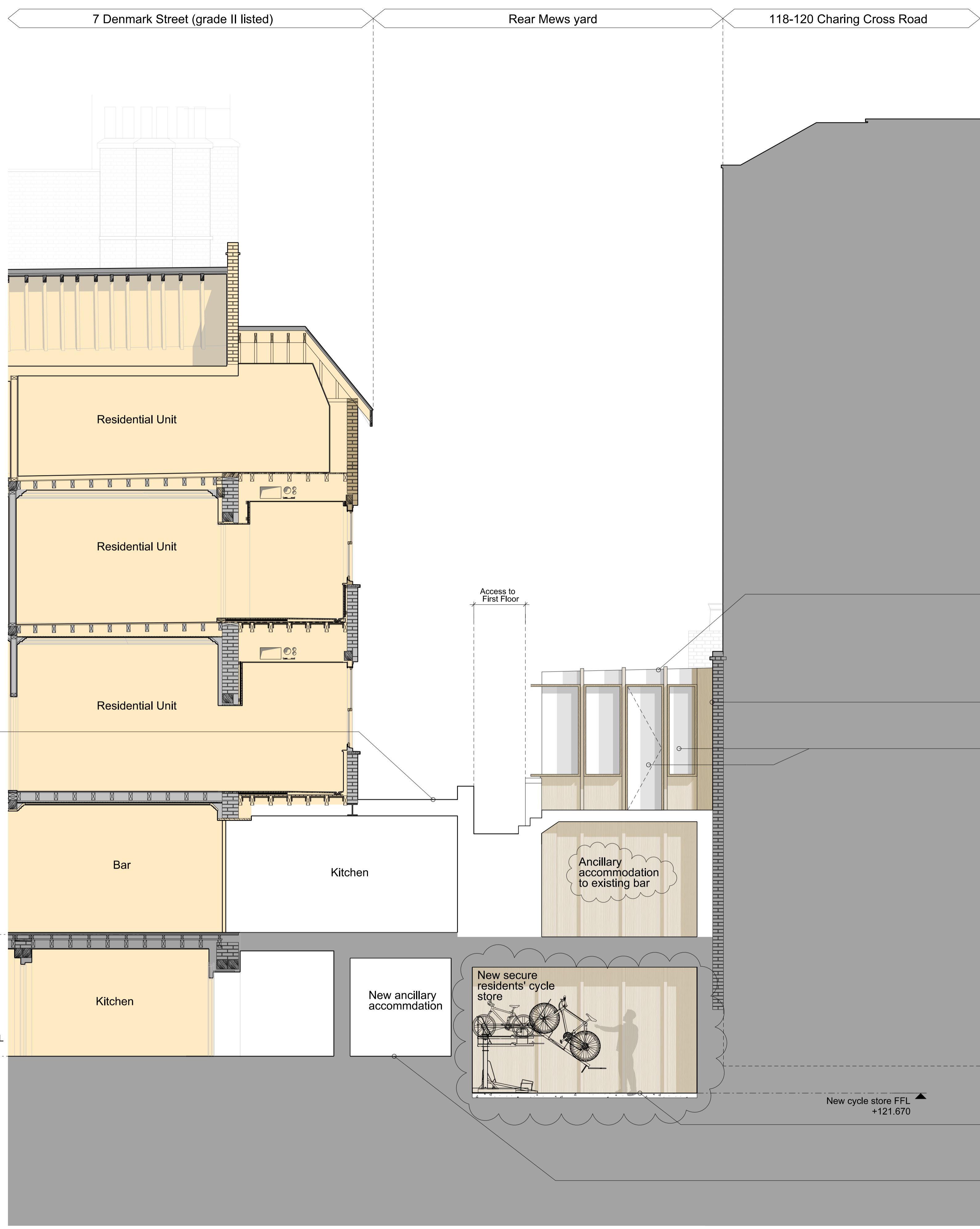
01 Proposed Section - Main House + Mews 7D(PL)16 Looking East 1:50
