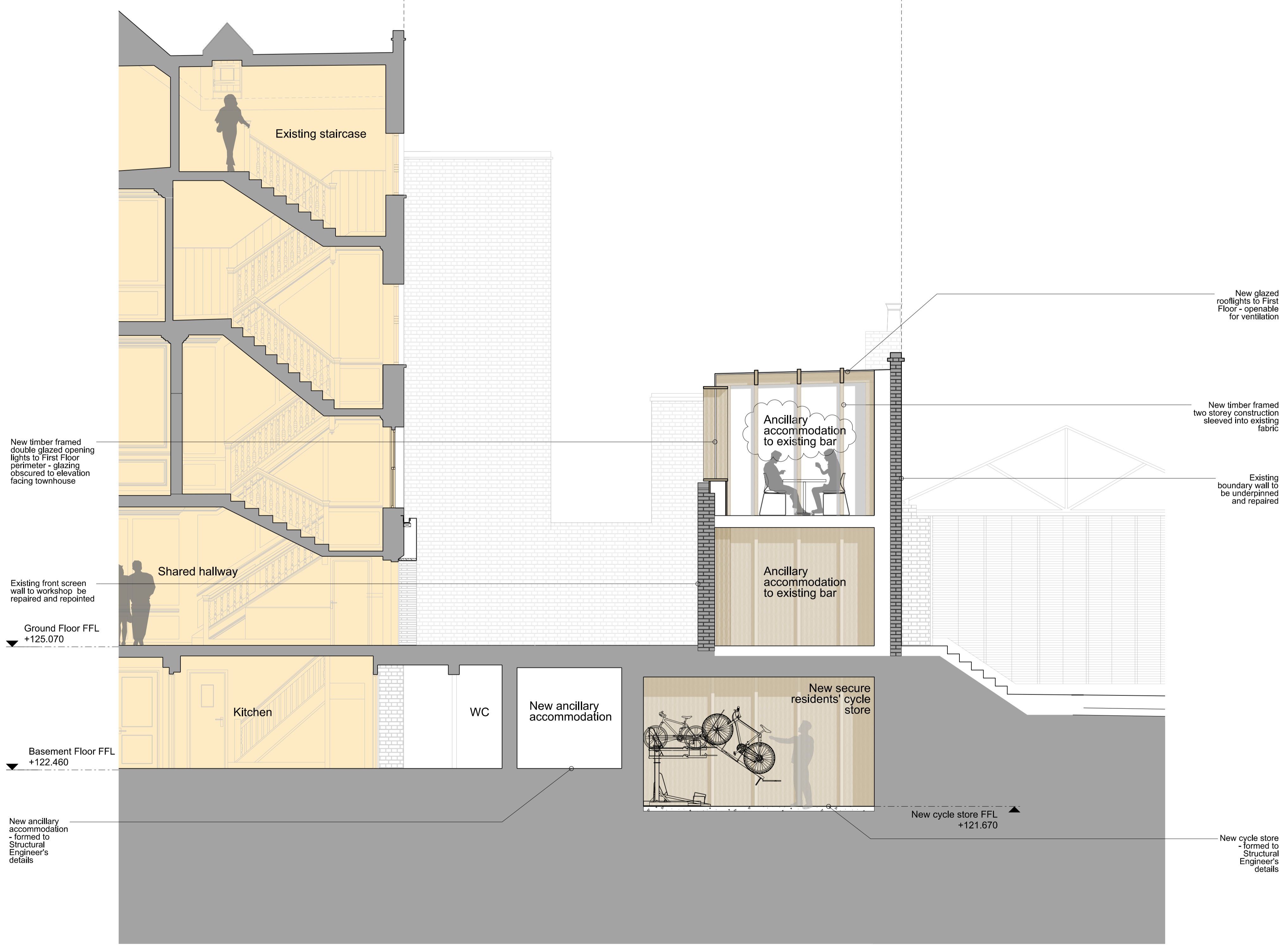
01 Proposed Section - Main House + Mews Looking East 1:50 7D(PL)12
