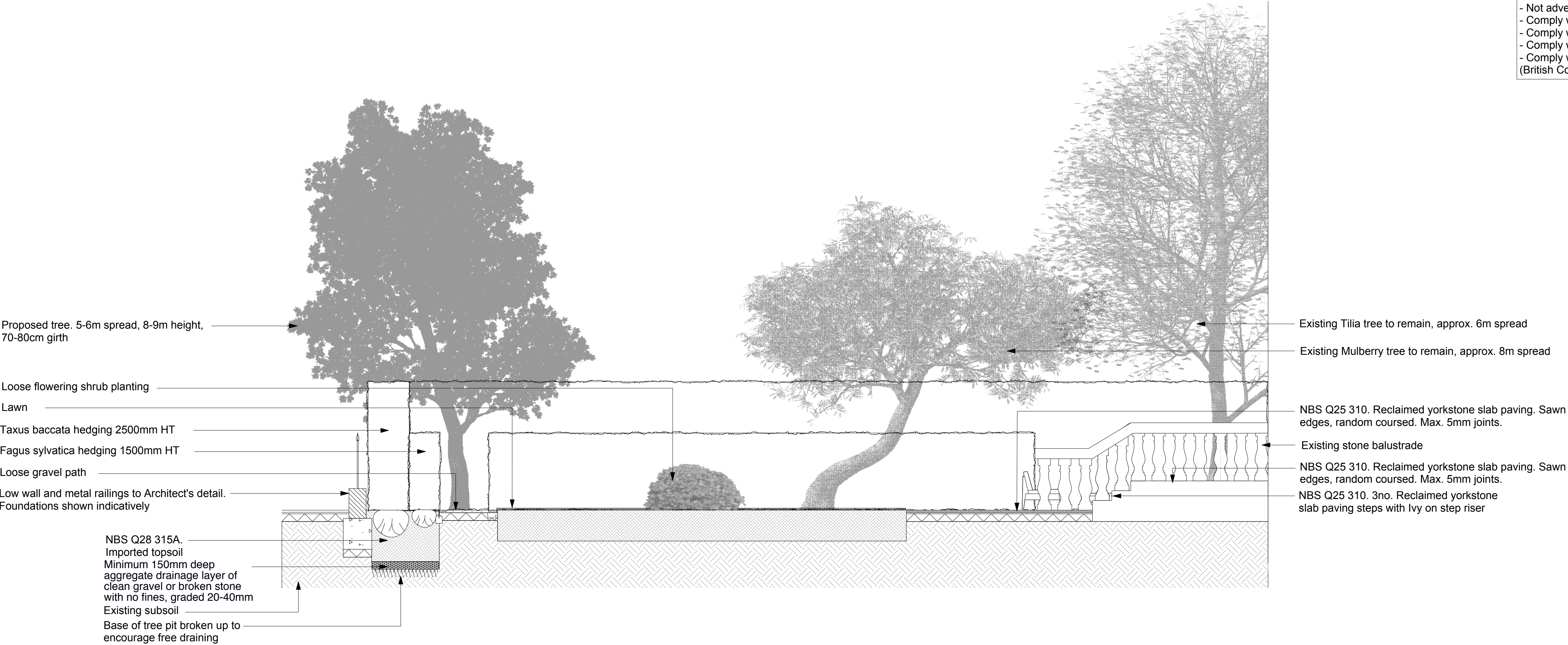
001 SECTIONAL ELEVATION AA Rear Garden 1:50 @ A1
