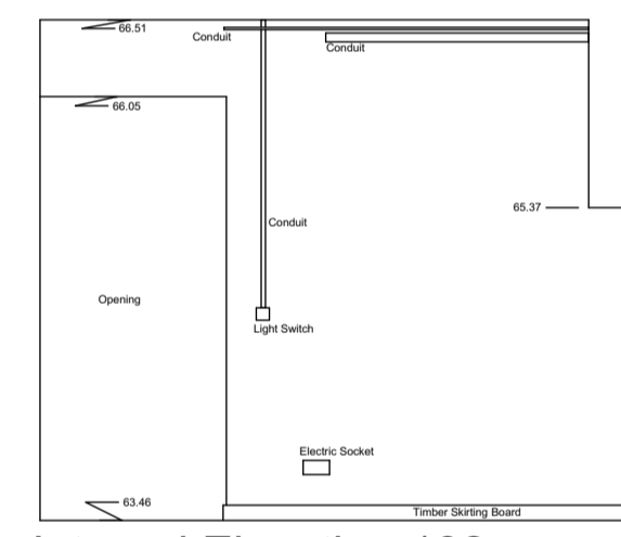
Internal Elevation 182 Datum 63.00m
