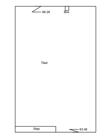
Internal Elevation 169 Datum 63.00m
