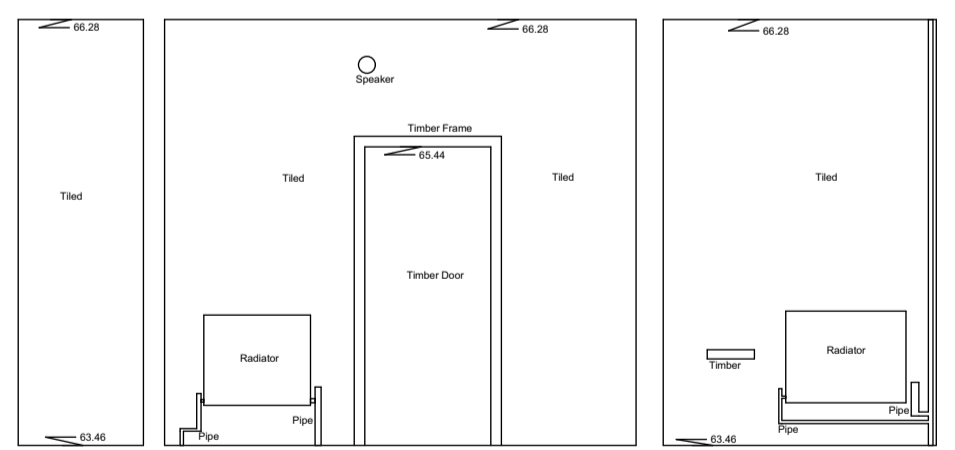
Internal Elevation 184 Datum 63.00m
