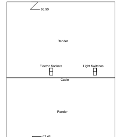
Internal Elevation 173 Datum 63.00m
