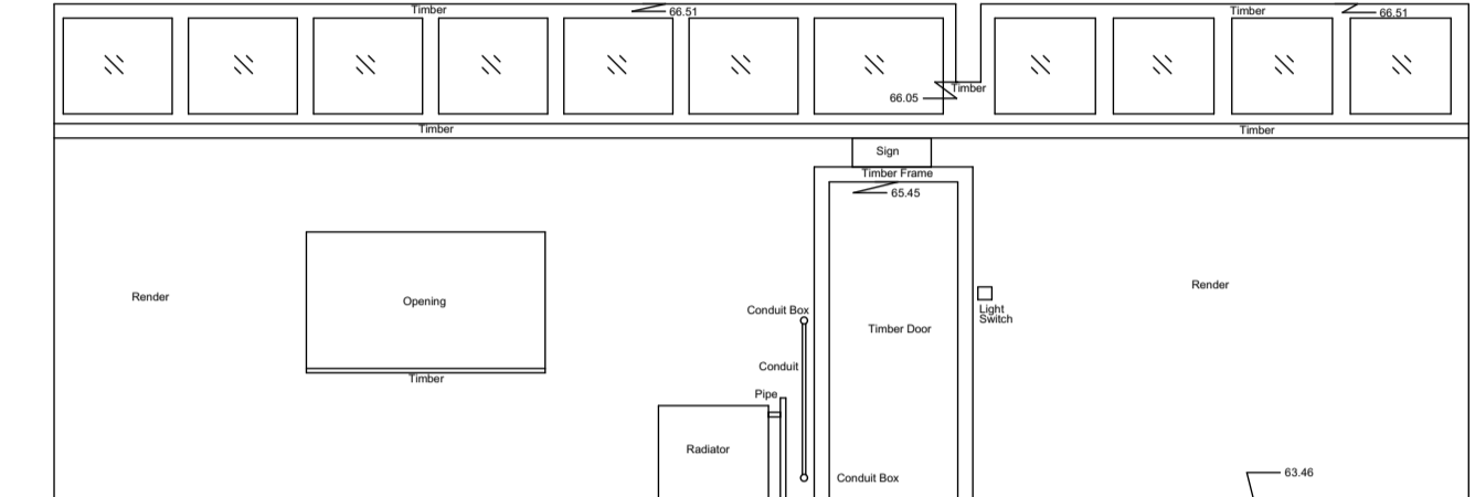
Internal Elevation 177 Datum 63.00m
