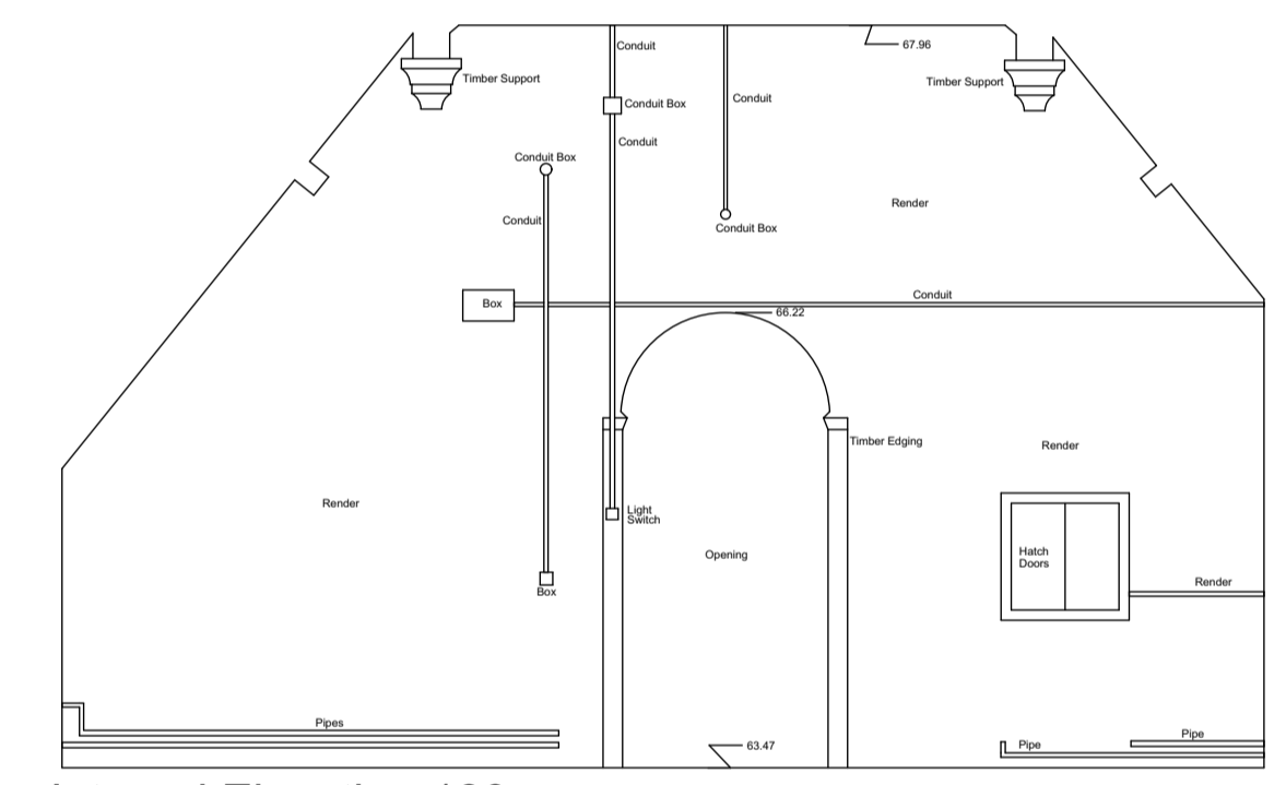
Internal Elevation 180 Datum 63.00m
