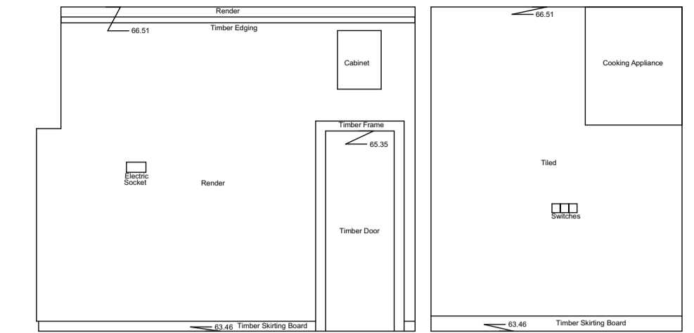
Internal Elevation 172 Datum 63.00m
