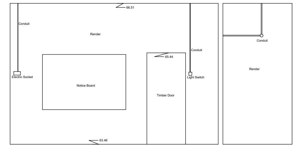
Internal Elevation 171 Datum 63.00m
