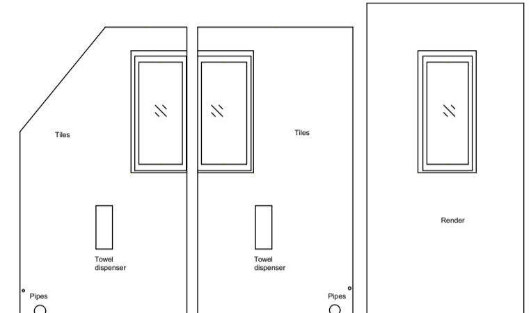
Internal Elevation 174 Datum 63.00m
