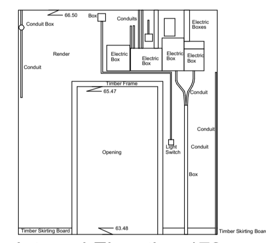
Internal Elevation 179 Datum 63.00m
