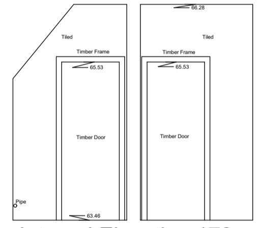
Internal Elevation 178 Datum 63.00m
