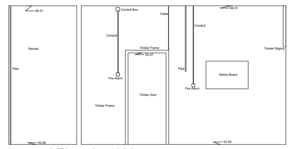
Internal Elevation 183 Datum 63.00m
