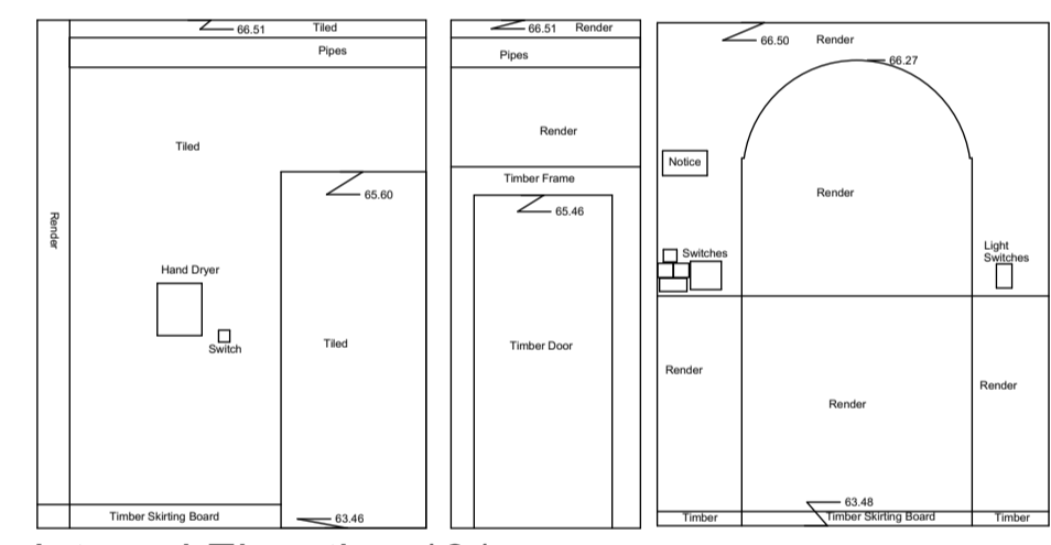
Internal Elevation 181 Datum 63.00m
