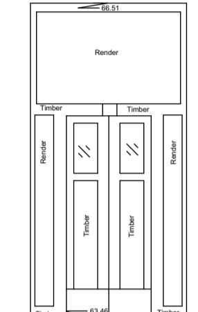
Internal Elevation 176 Datum 63.00m
