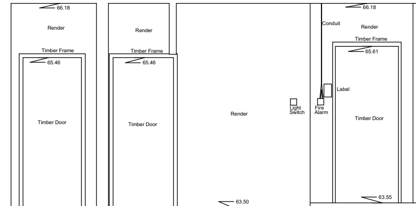
Internal Elevation 152 Datum 63.00m
