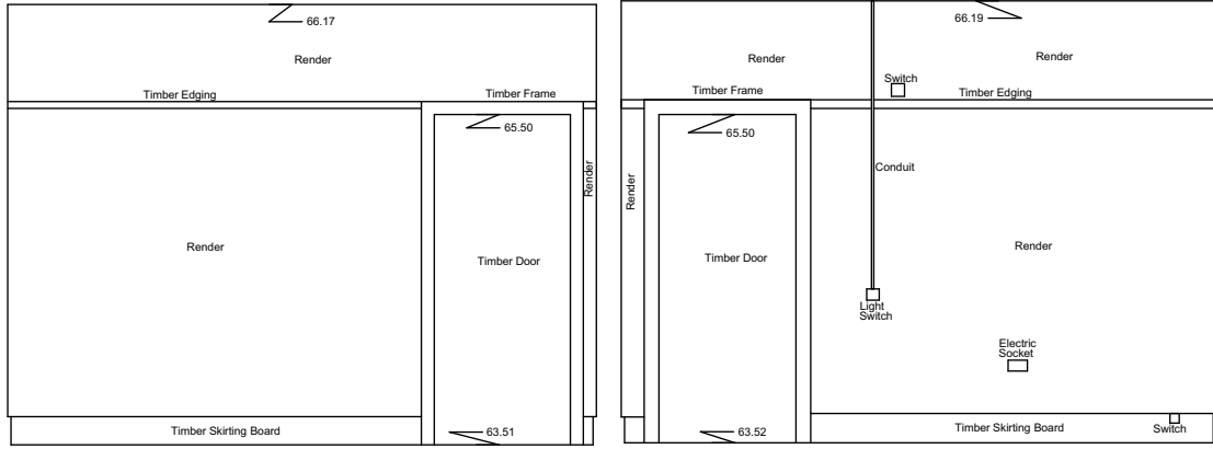
Internal Elevation 154 Datum 63.00m
