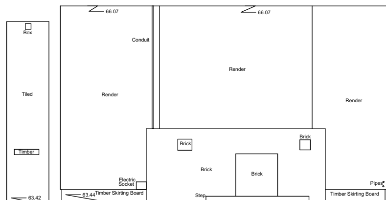
Internal Elevation 163 Datum 63.00m
