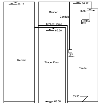
Internal Elevation 149 Datum 63.00m
