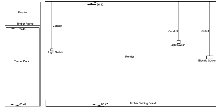
Internal Elevation 160A Datum 63.00m
