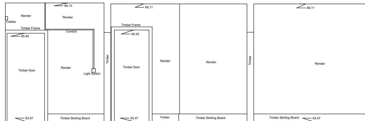
Internal Elevation 156 Datum 63.00m
