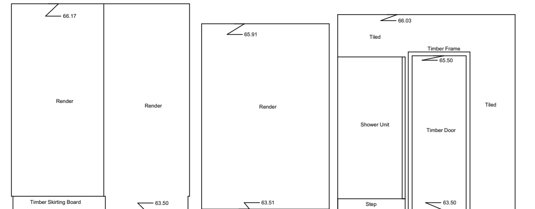
Internal Elevation 153 Datum 63.00m
