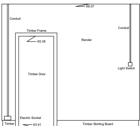
Internal Elevation 159 Datum 63.00m
