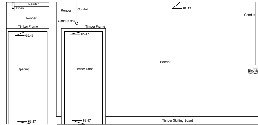
Internal Elevation 161 Datum 63.00m
