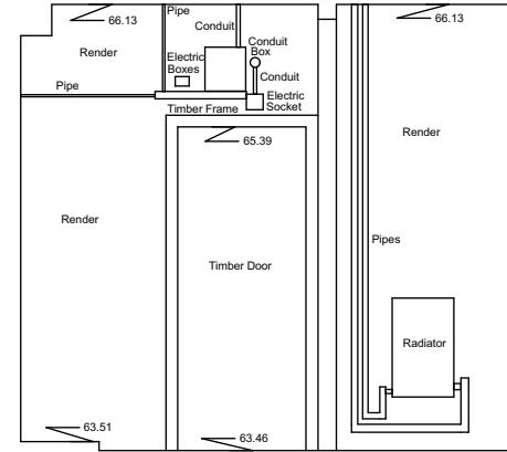
Internal Elevation 165 Datum 63.00m
