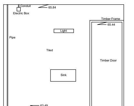
Internal Elevation 162A Datum 63.00m
