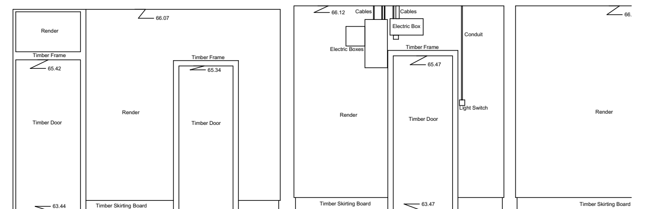
Internal Elevation 157 Datum 63.00m
