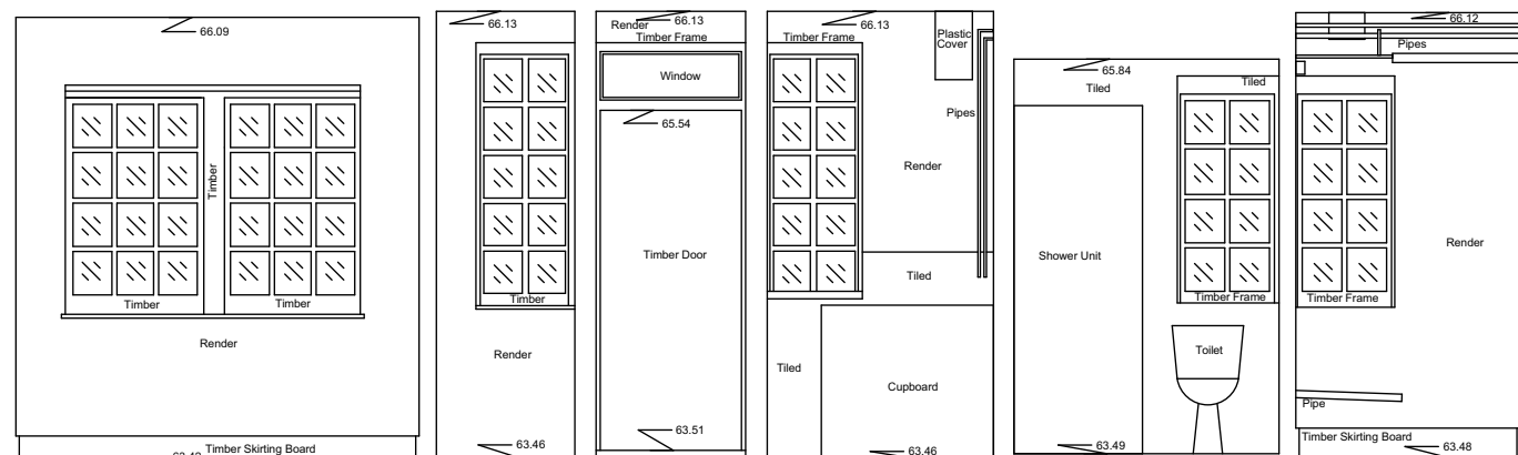
Internal Elevation 155 Datum 63.00m
