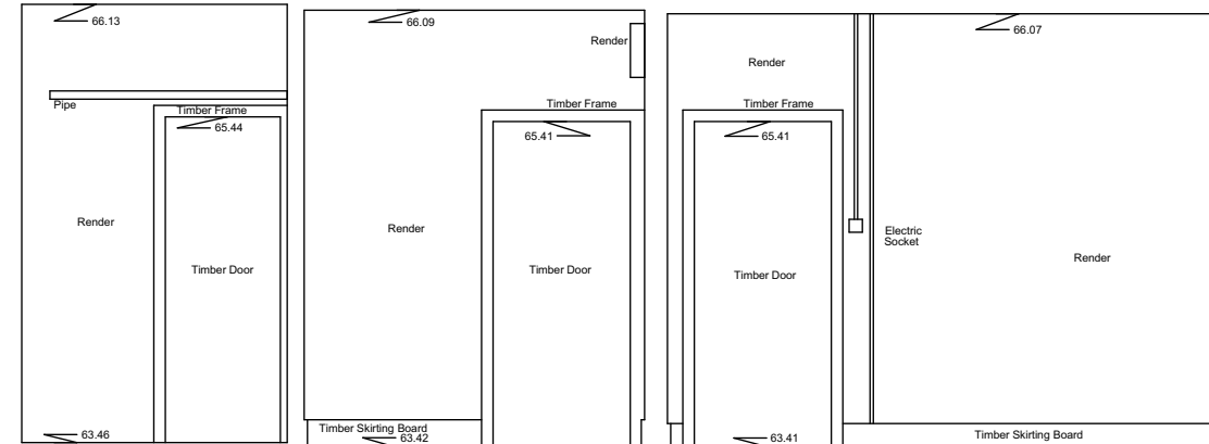
Internal Elevation 166 Datum 63.00m
