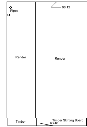
Internal Elevation 162 Datum 63.00m
