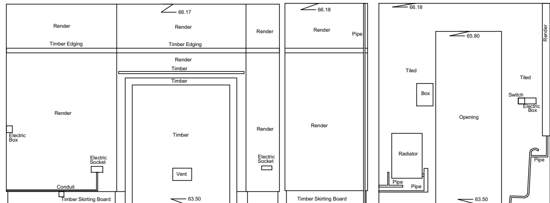
Internal Elevation 151 Datum 63.00m
