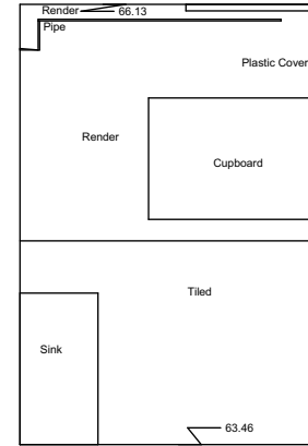
Internal Elevation 164 Datum 63.00m
