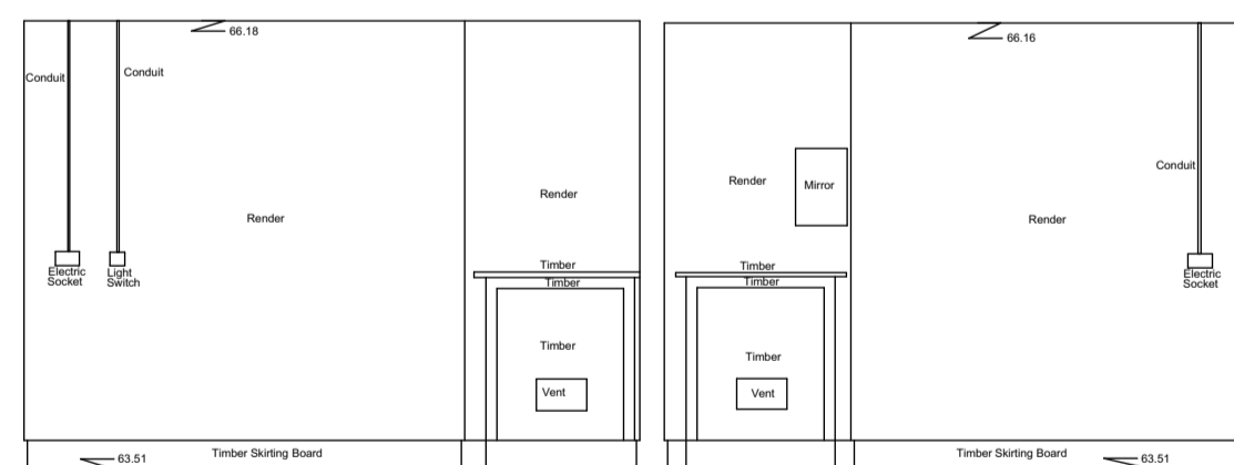
Internal Elevation 144 Datum 63.00m
