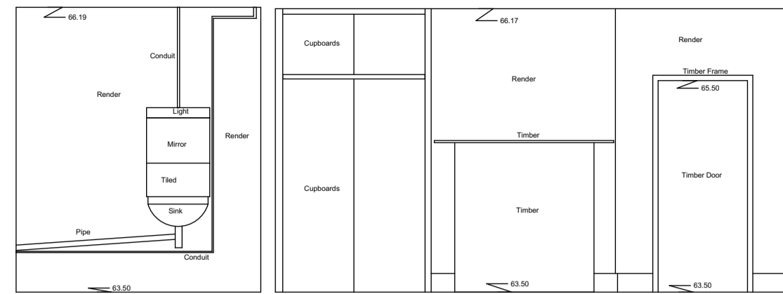
Internal Elevation 133 Datum 63.00m
