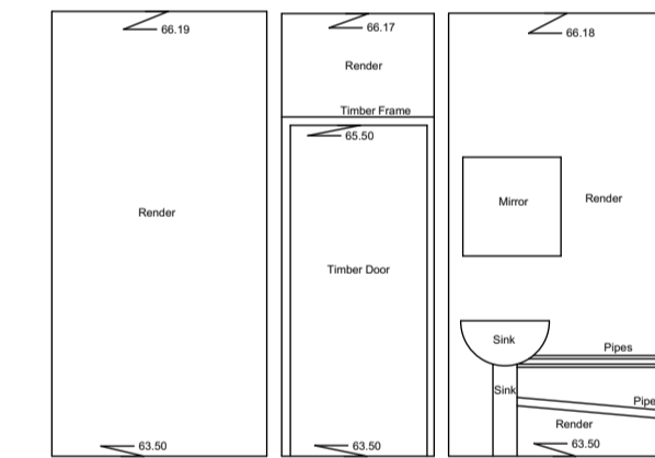
Internal Elevation 142 Datum 63.00m
