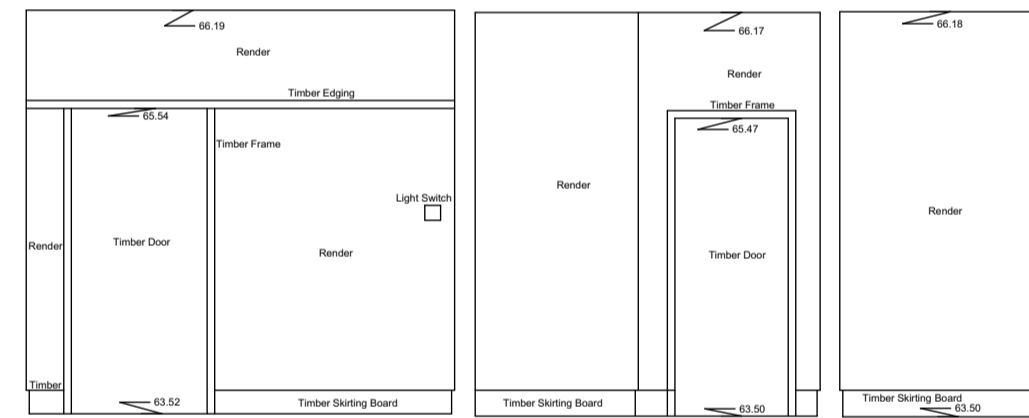
Internal Elevation 139 Datum 63.00m
