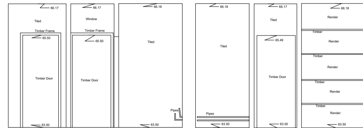
Internal Elevation 140 Datum 63.00m
