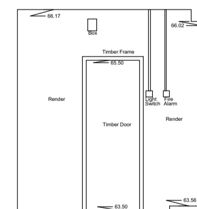
Internal Elevation 146 Datum 63.00m
