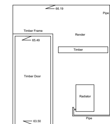
Internal Elevation 146A Datum 63.00m
