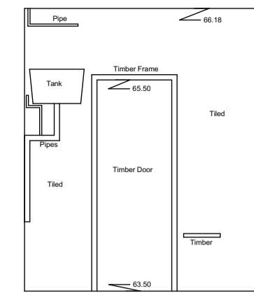
Internal Elevation 135 Datum 63.00m
