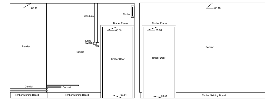
Internal Elevation 136 Datum 63.00m
