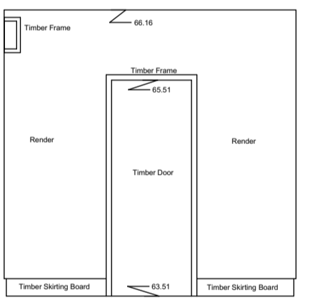
Internal Elevation 143 Datum 63.00m
