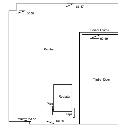
Internal Elevation 134 Datum 63.00m
