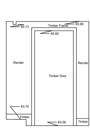
Internal Elevation 138 Datum 63.00m
