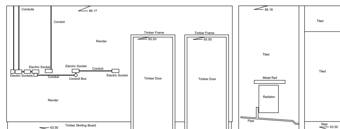
Internal Elevation 145 Datum 63.00m
