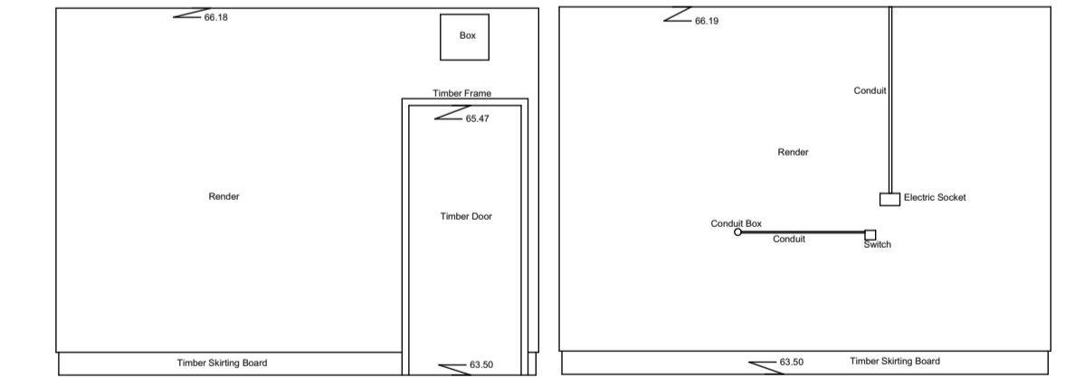
Internal Elevation 132 Datum 63.00m
