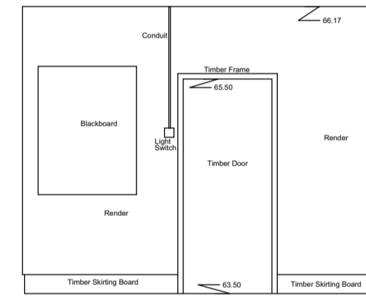
Internal Elevation 122 Datum 63.00m
