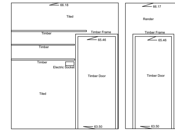
Internal Elevation 128 Datum 63.00m
