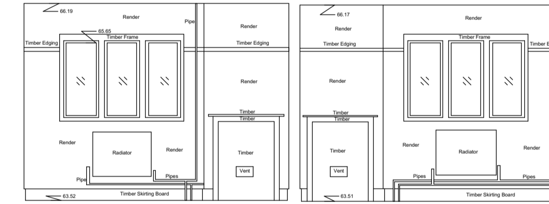
Internal Elevation 124 Datum 63.00m
