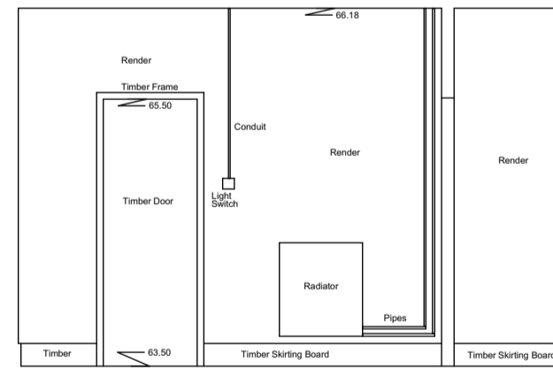
Internal Elevation 127 Datum 63.00m
