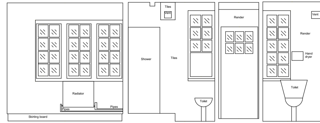
Internal Elevation 114 Datum 63.00m
