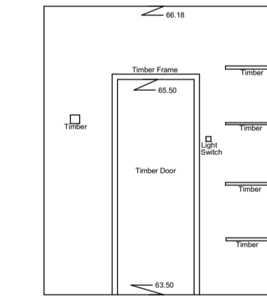
Internal Elevation 131 Datum 63.00m
