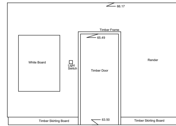
Internal Elevation 120 Datum 63.00m
