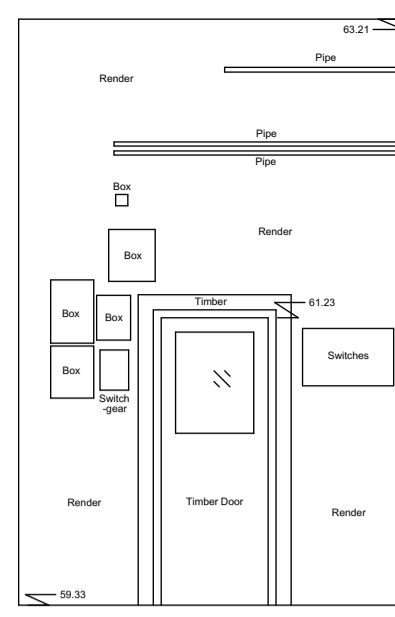
Internal Elevation 108 Datum 58.00m
