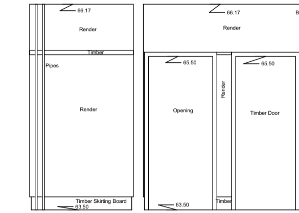
Internal Elevation 117 Datum 63.00m
