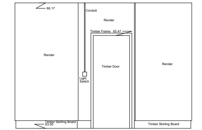
Internal Elevation 118 Datum 63.00m
