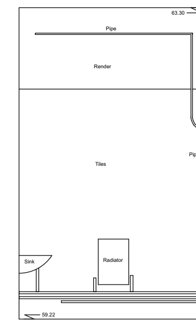
Internal Elevation 111 Datum 58.00m
