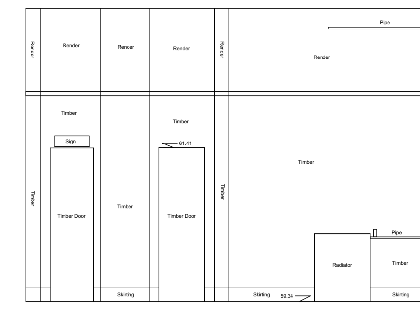
Internal Elevation 113 Datum 58.00m
