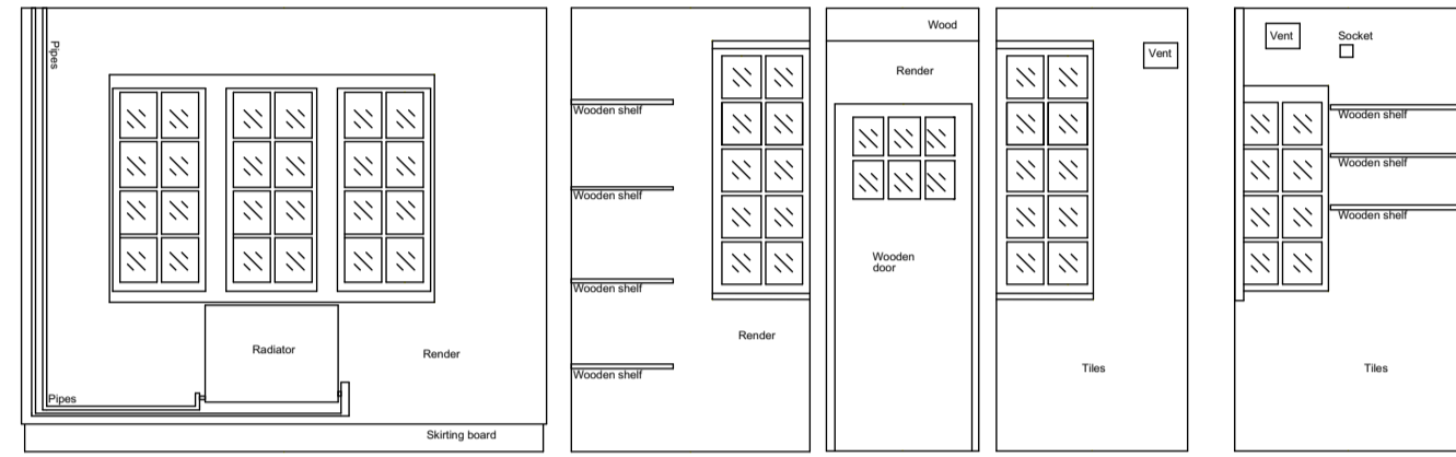
Internal Elevation 109 Datum 58.00m
