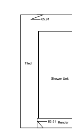
Internal Elevation 116 Datum 63.00m
