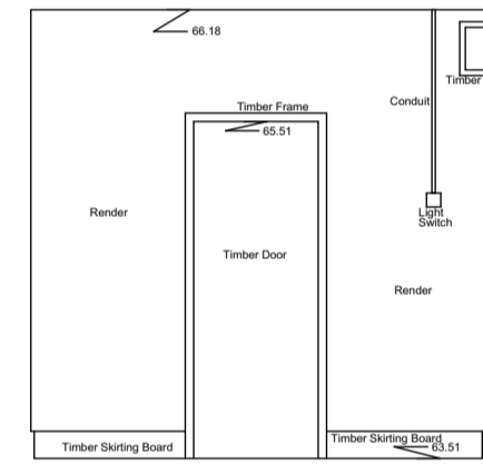
Internal Elevation 121 Datum 63.00m
