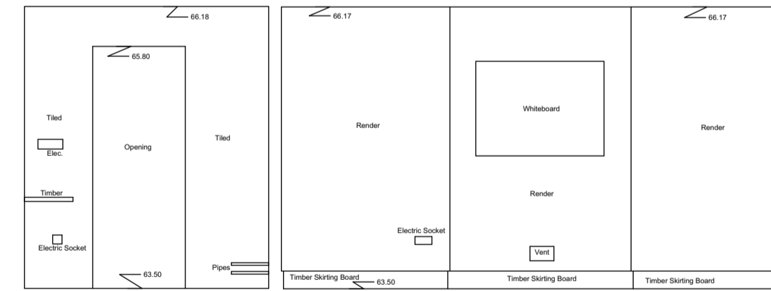
Internal Elevation 129 Datum 63.00m
