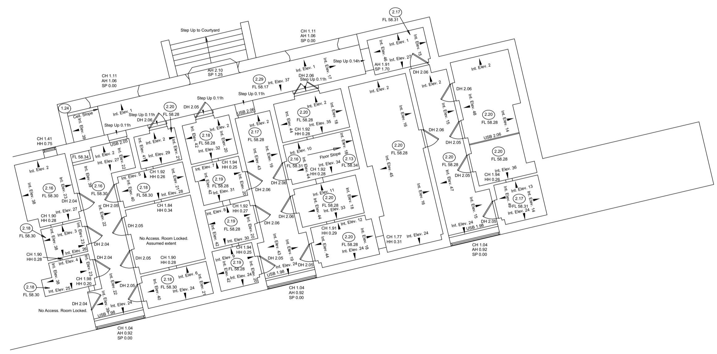
Basement Plan
