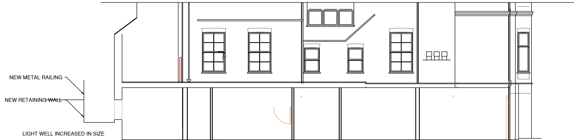
PART SECTION AS PROPOSED
