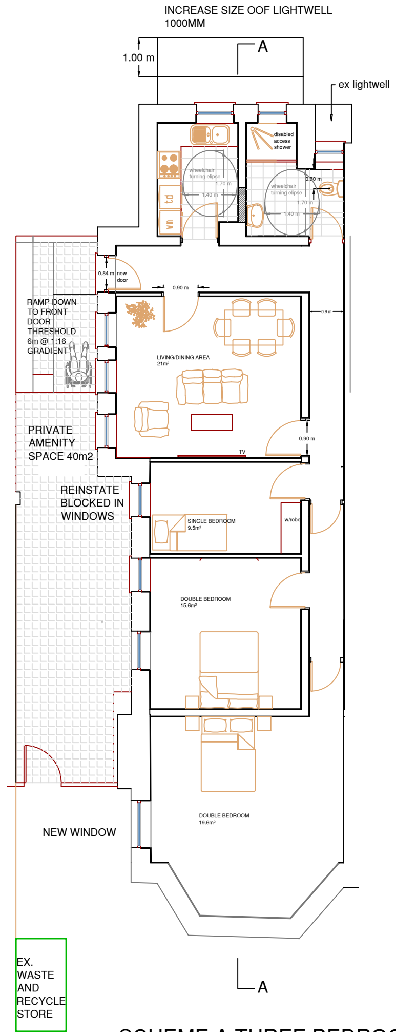
SCHEME A THREE BEDROOM FLOOR PLAN AS PROPOSED
