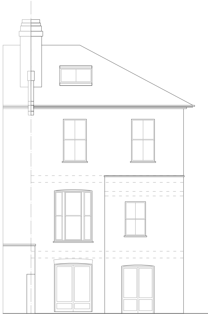
REAR ELEVATION E: 1/100
