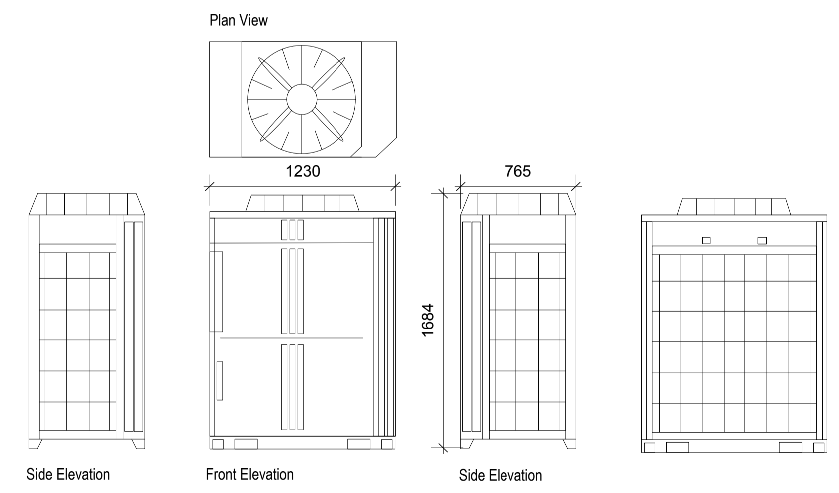
3 CONDENSER UNIT ELEVATIONS 1:25
