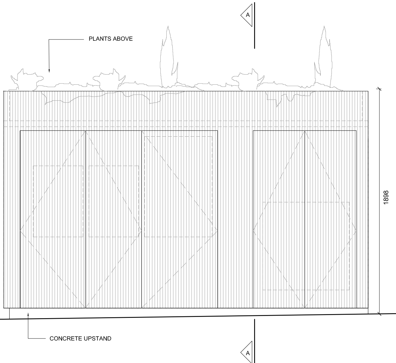
SIDE ELEVATION
