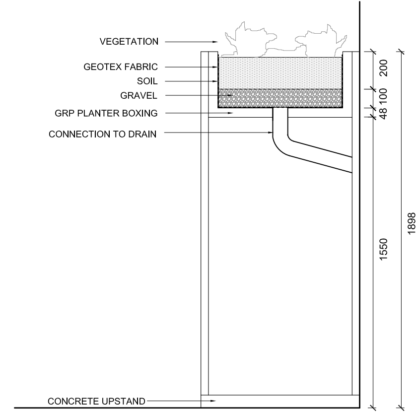
SECTION A
