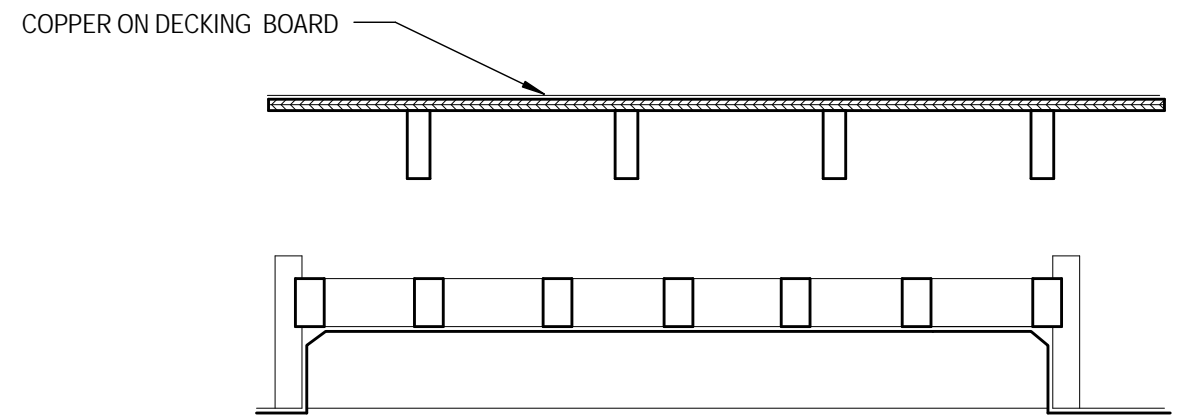
EXISTING TYPICAL SECTION A - A
