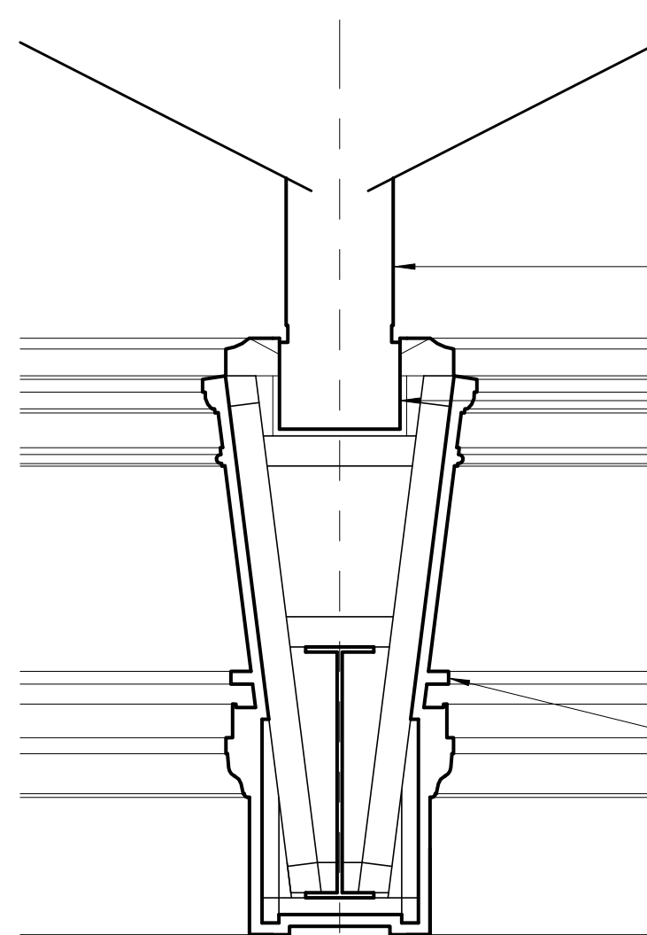
EXISTING SECTION THROUGH GIRDER
