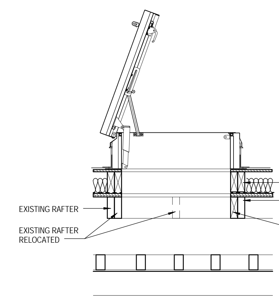
PROPOSED SECTION B - B THROUGH HATCH
