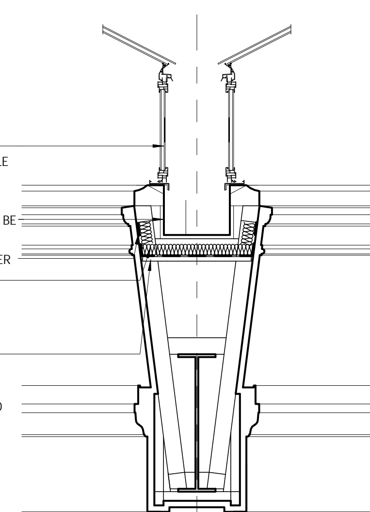
PROPOSED SECTION THROUGH GIRDER
