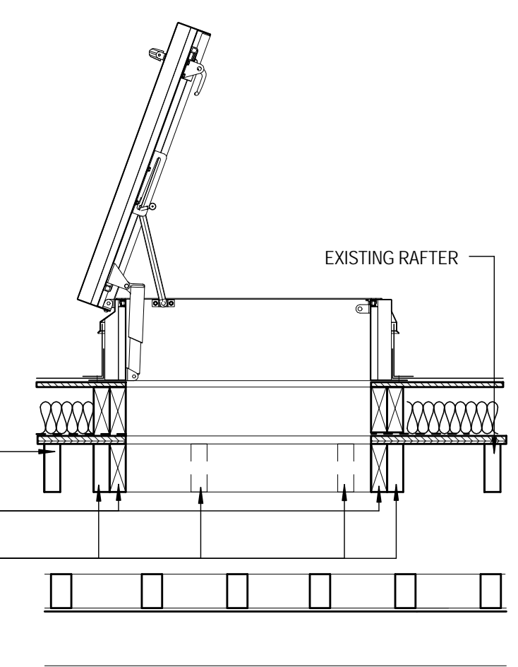
PROPOSED SECTION THROUGH HATCH WHERE 2 RAFTERS WILL BE RELOCATED
