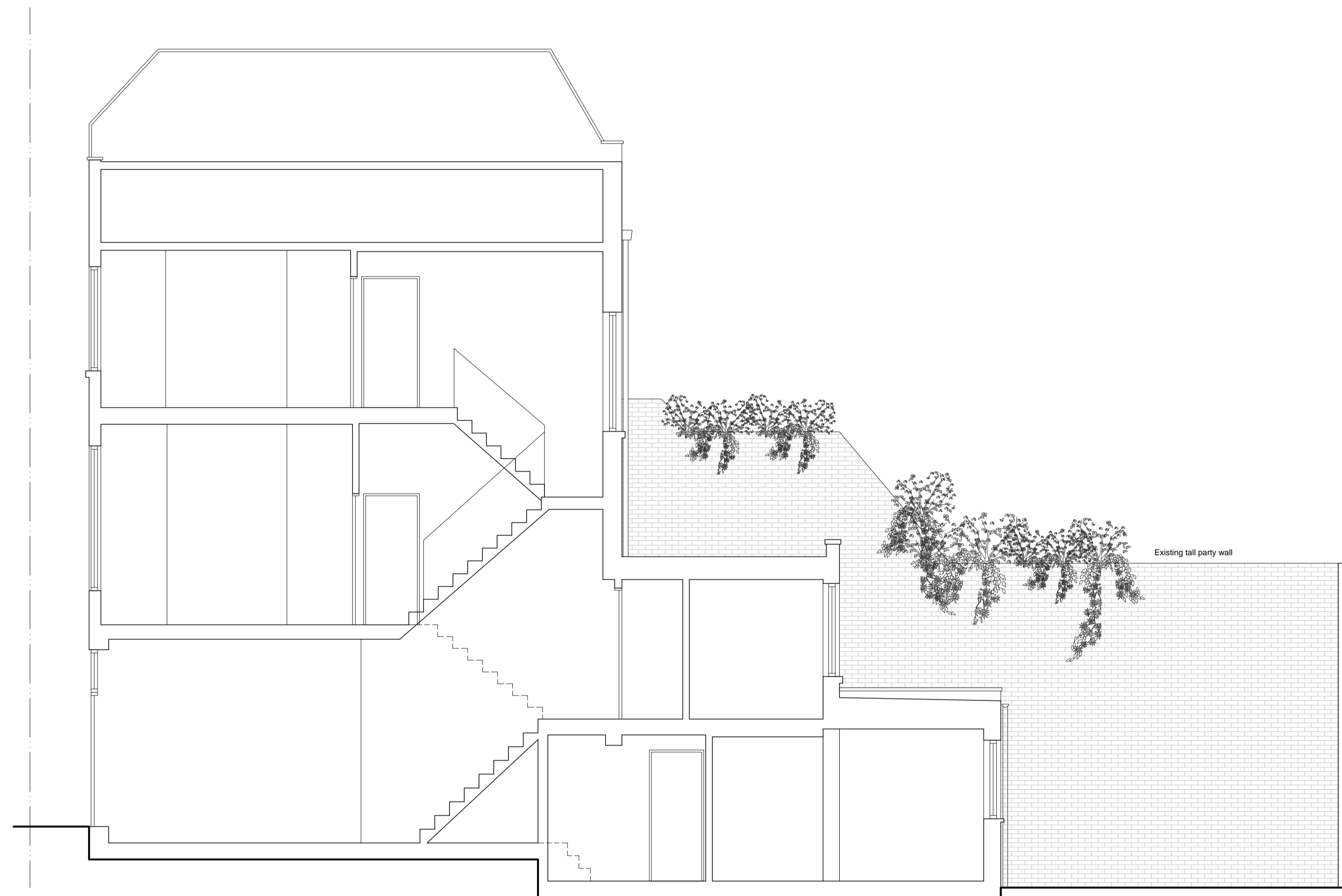
Existing Section Scale 1:50
