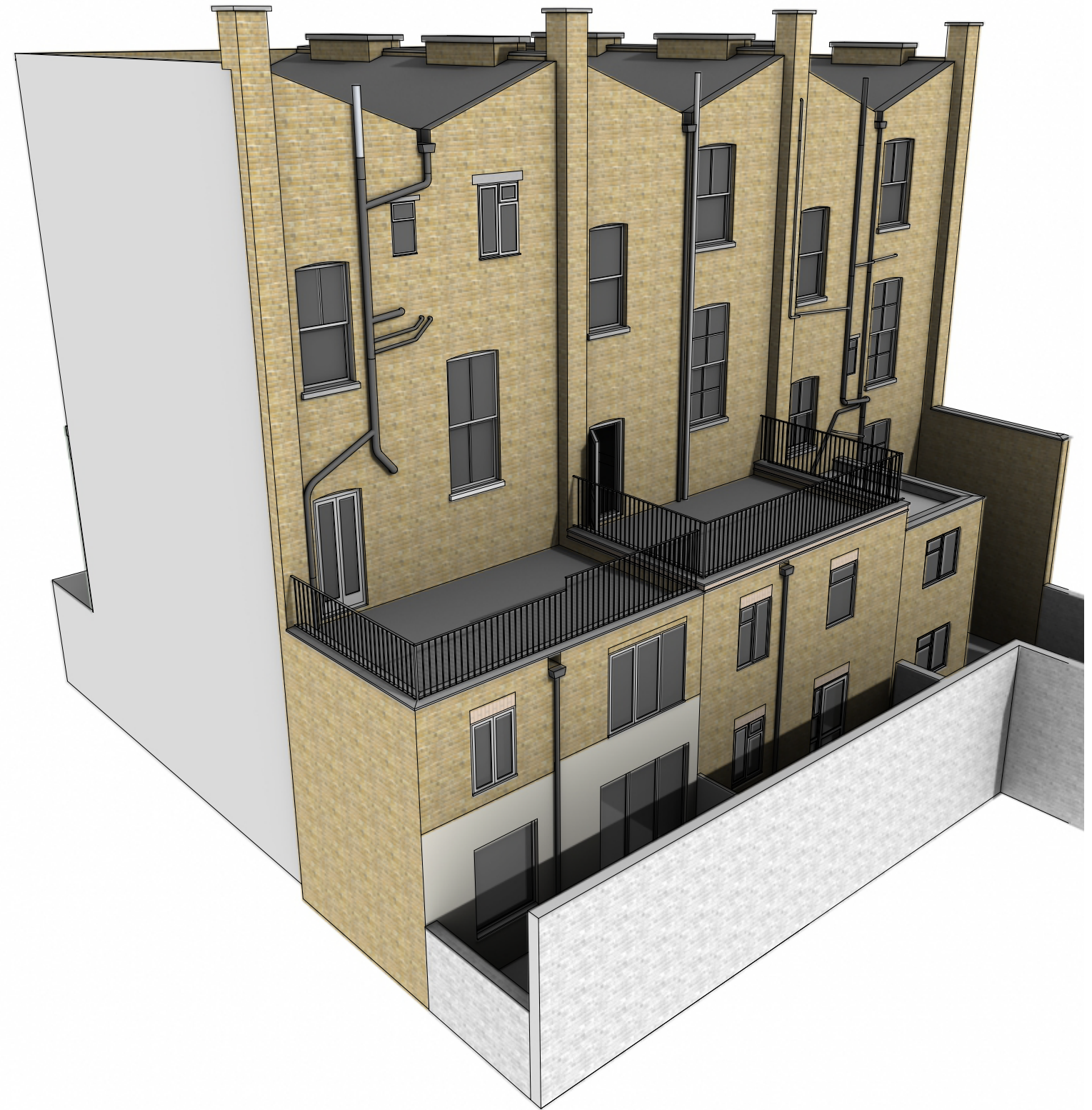
3.2 Rear Massing- Existing
