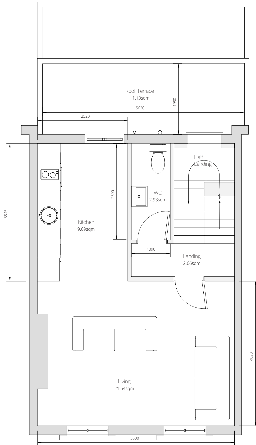
2nd Floor - Proposed
