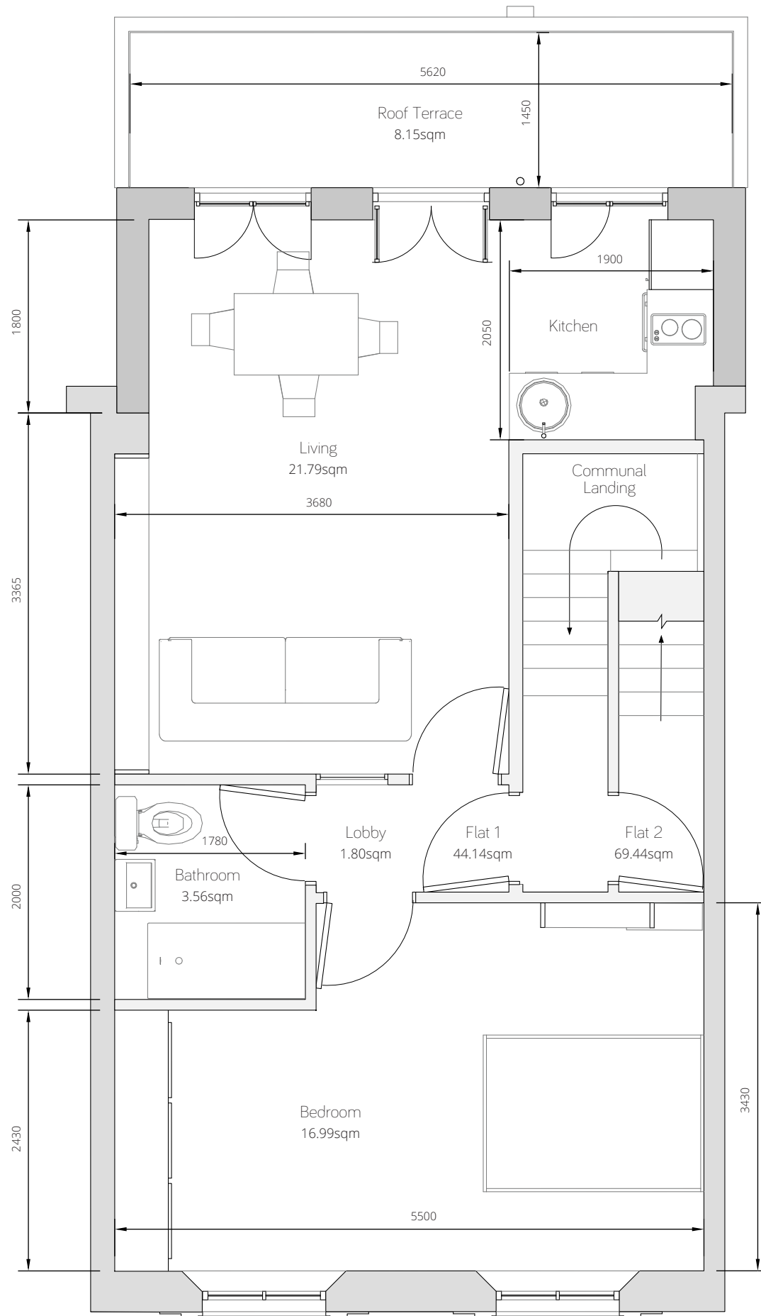
1st Floor - Proposed (9.49sqm additional)
