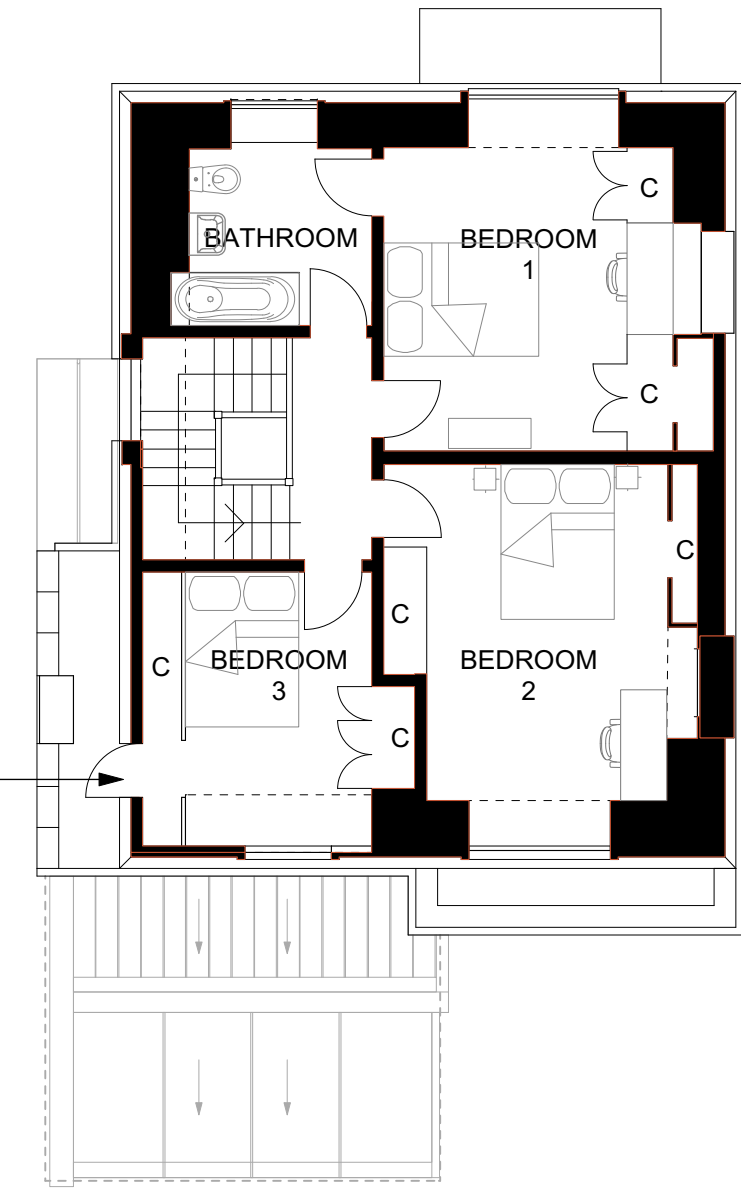
Proposed Second Floor Plan Scale 1:100
