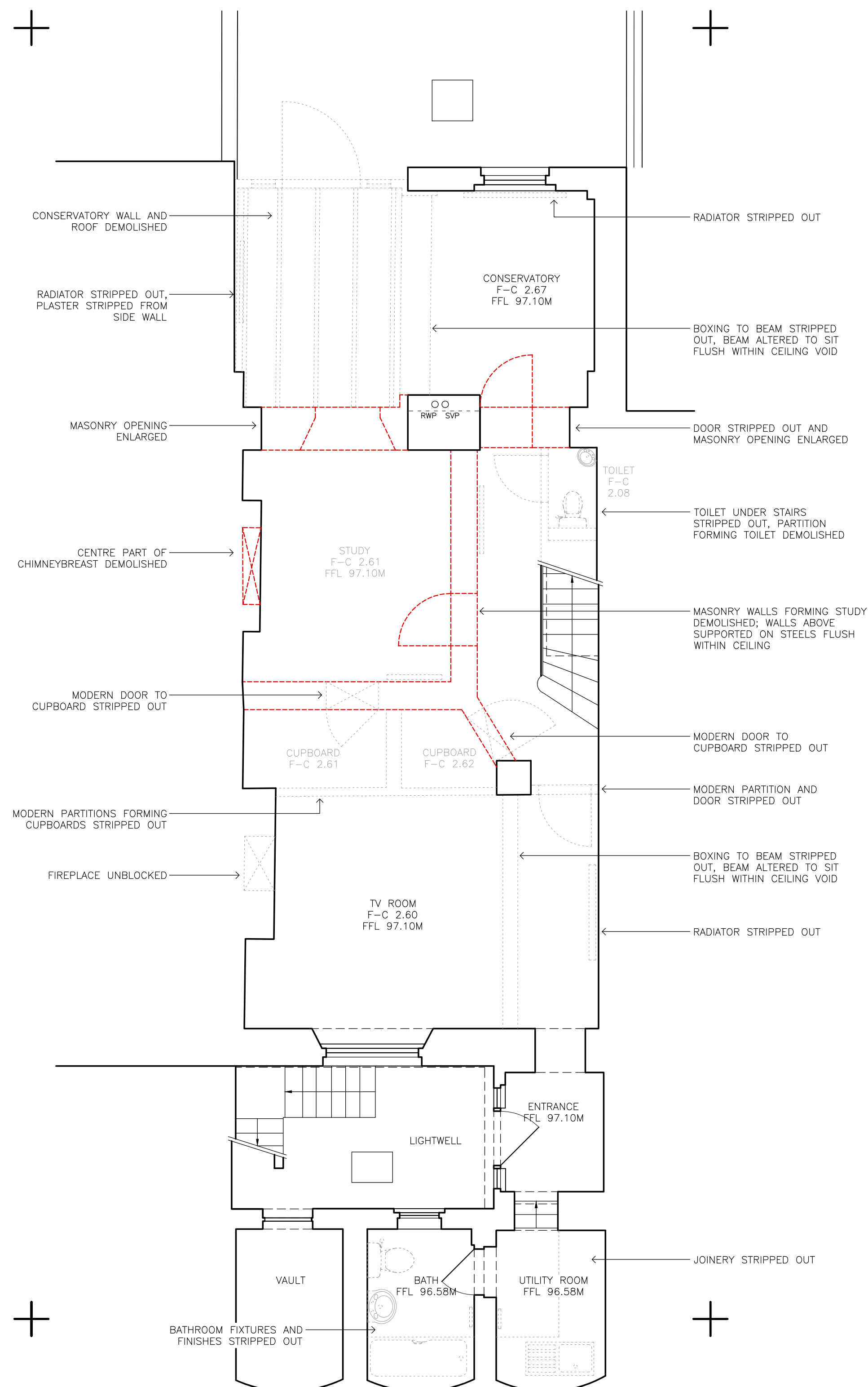
BASEMENT FLOOR PLAN
