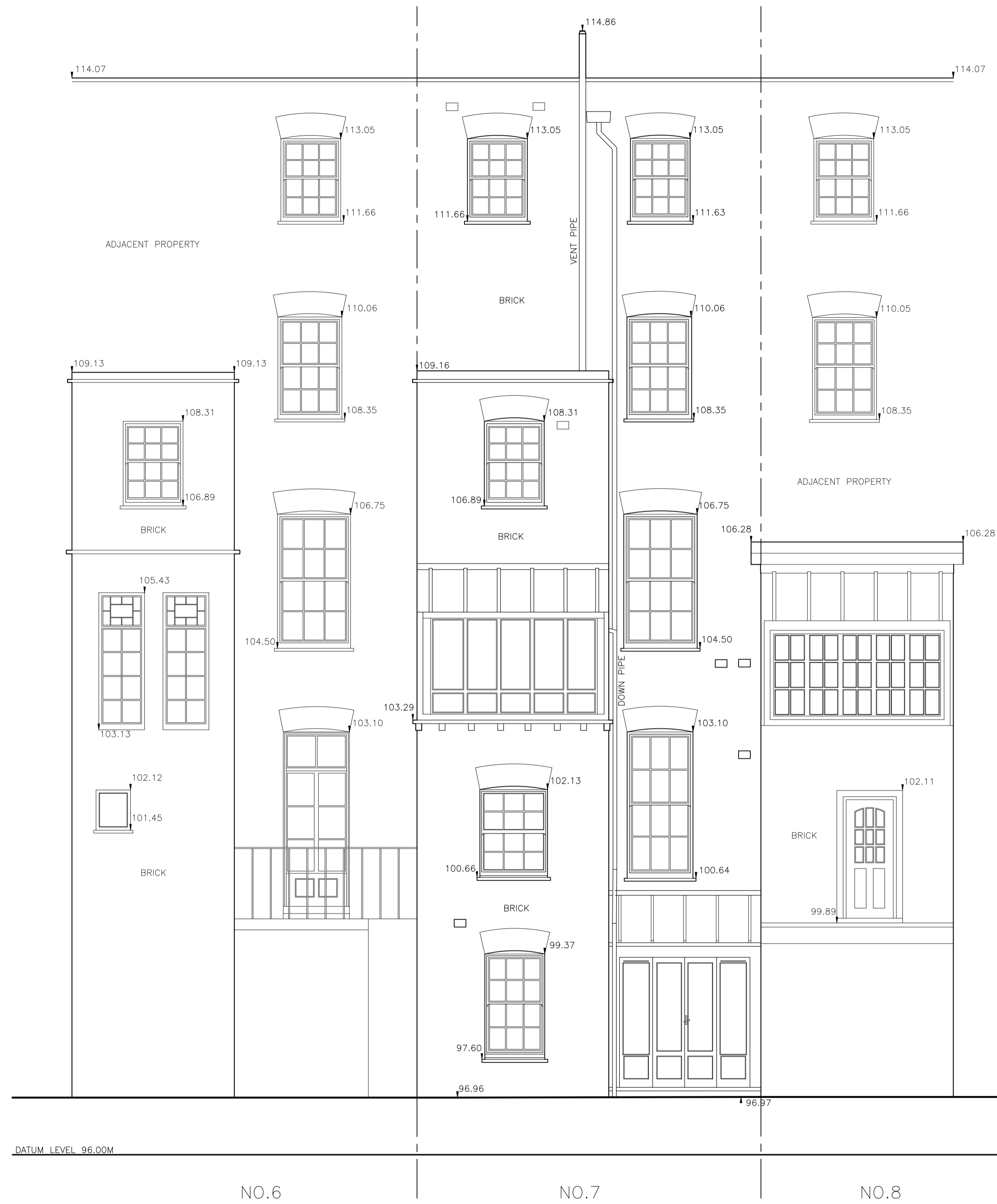
REAR ELEVATION
