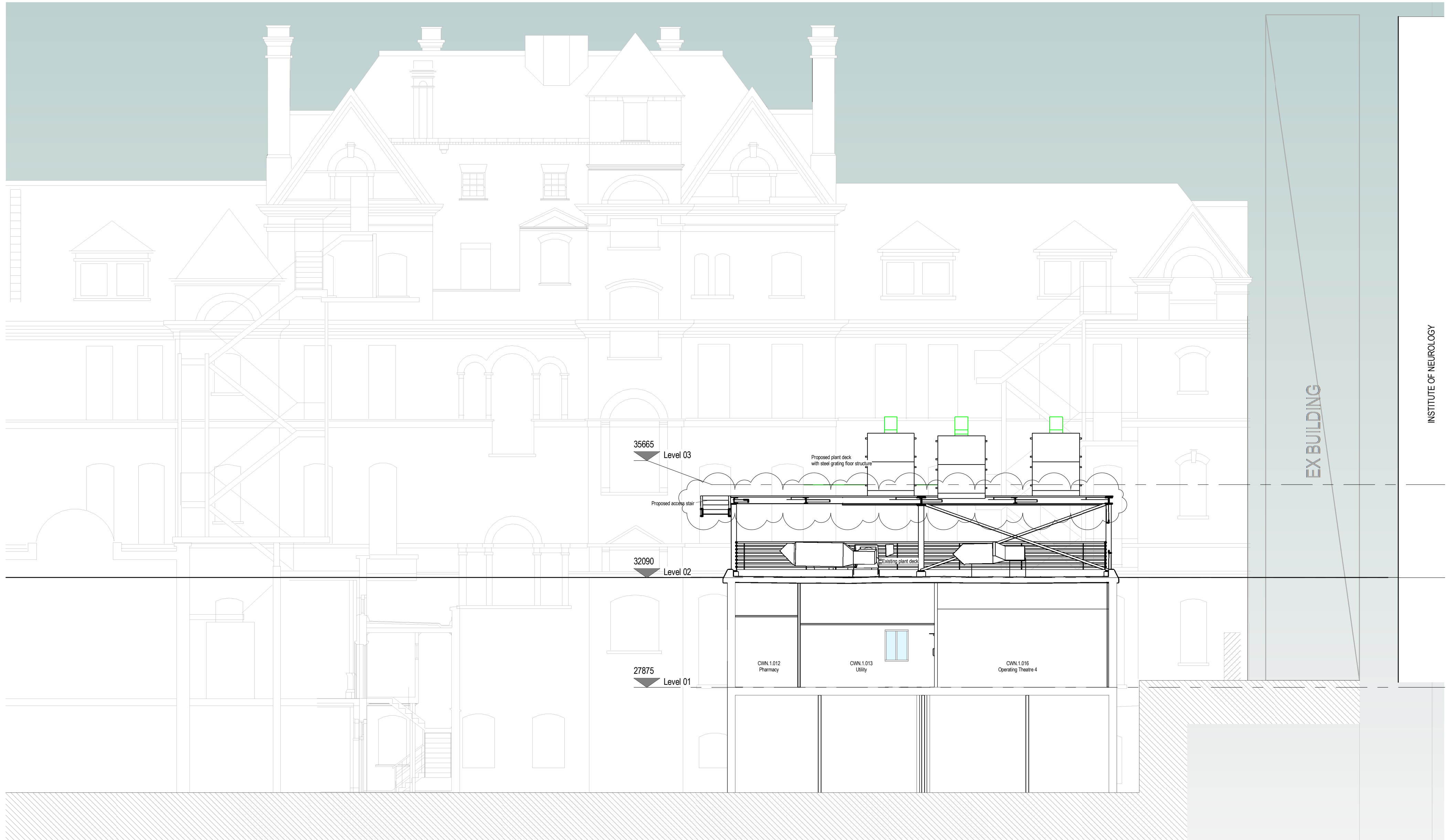
1 Proposed East Section - Albany Wing 1: 100
