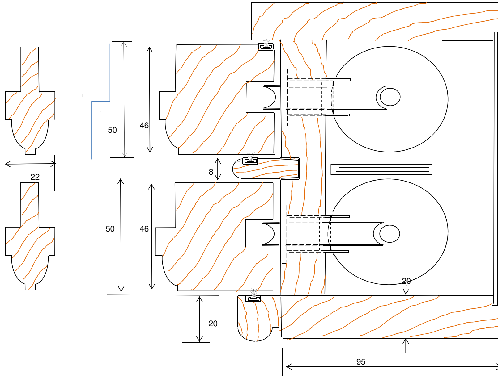
Section of Sash Stile Glazing Bar and Sash box
