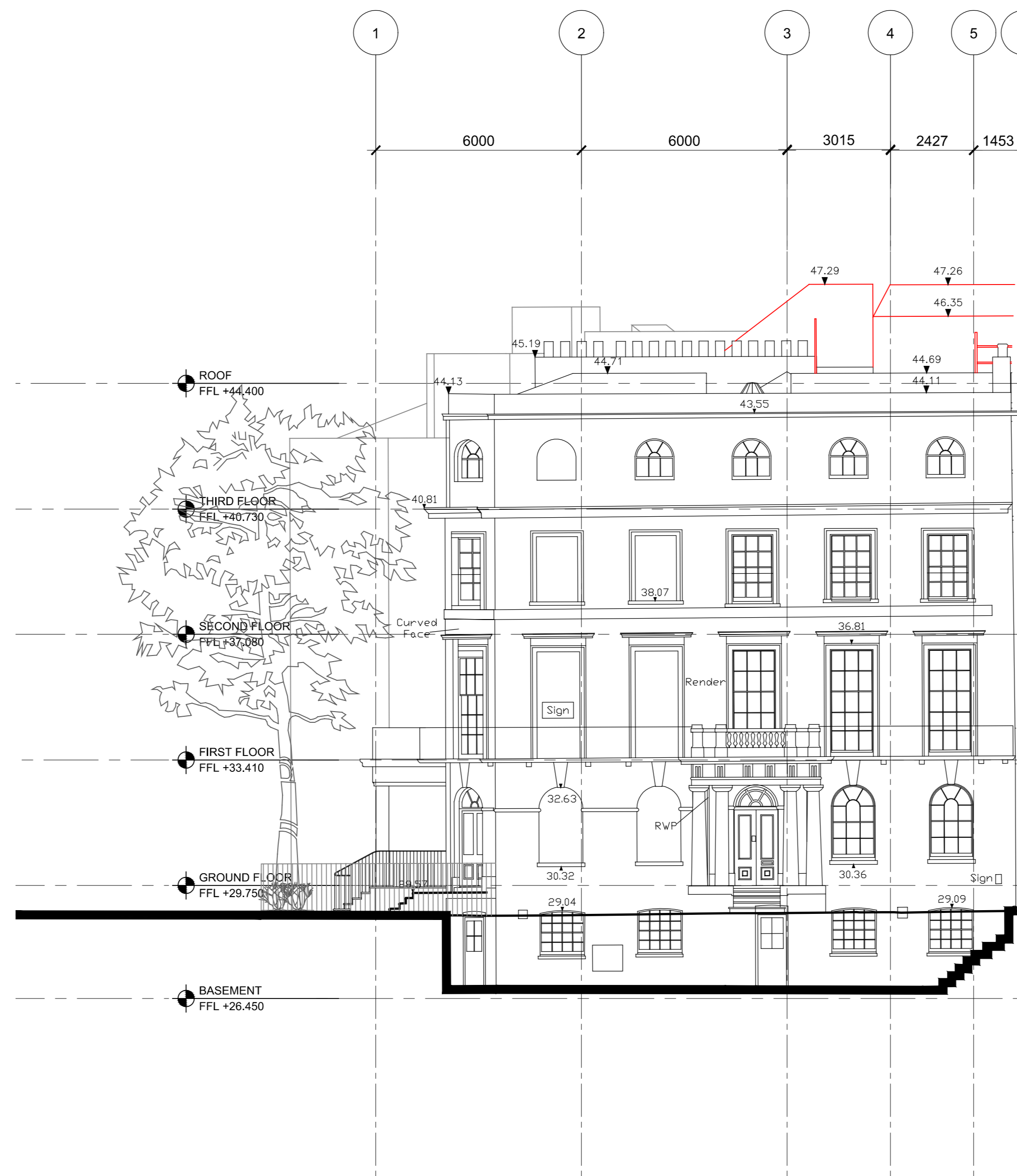
3 Albany Street Elevation - Demolition SCALE: 1:100 @ A0
