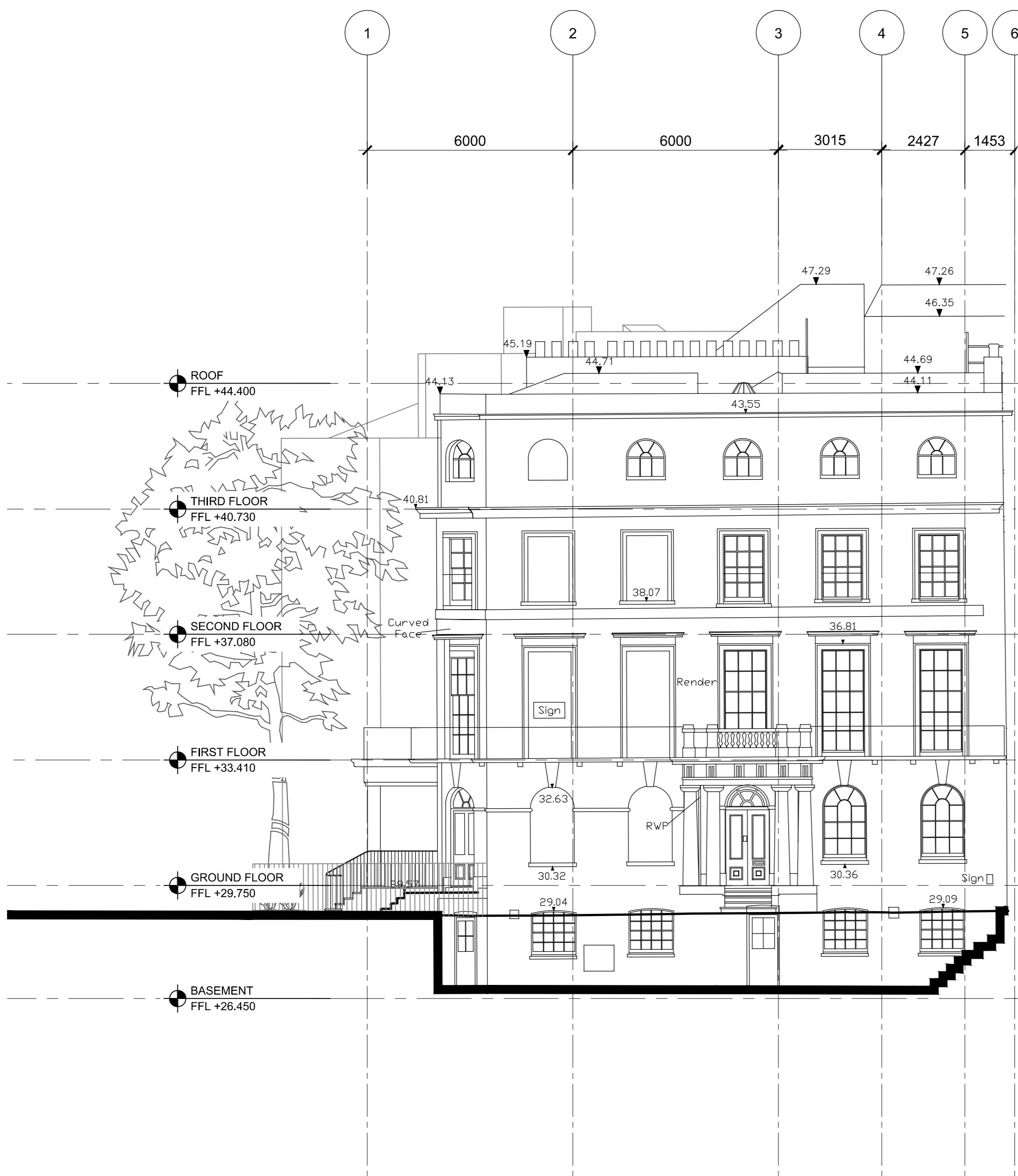
2 Albany Street Elevation - Existing SCALE: 1:100 @ A0
