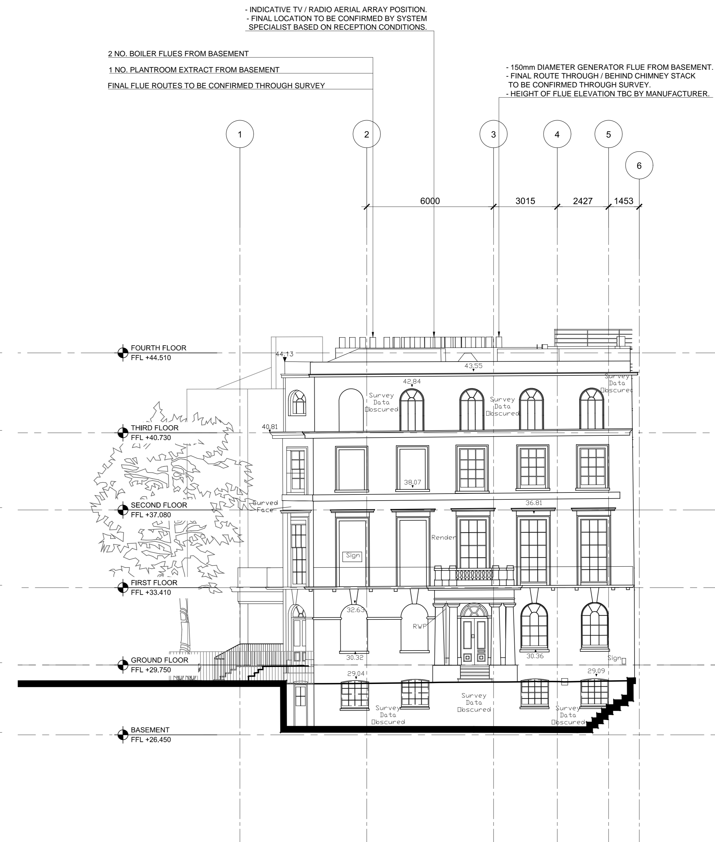
4 Albany Street Elevation - Proposed SCALE: 1:100 @ A0
