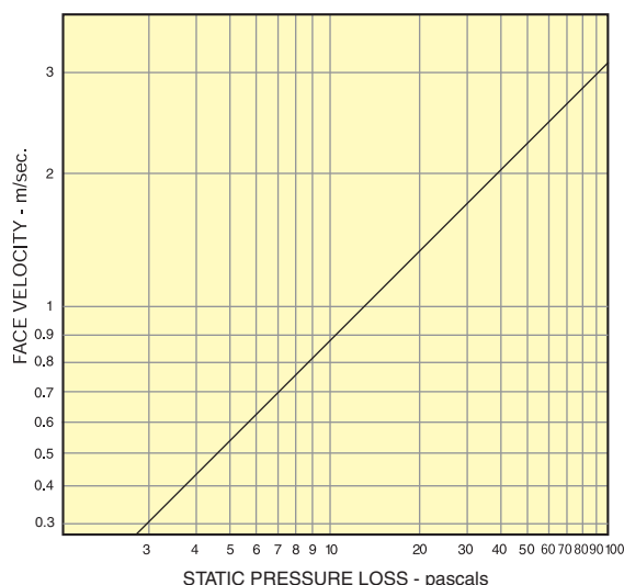
PRESSURE LOSS CHART FOR EMTEC LAAC 30 & LAAC 15 ACOUSTIC LOUVRES
