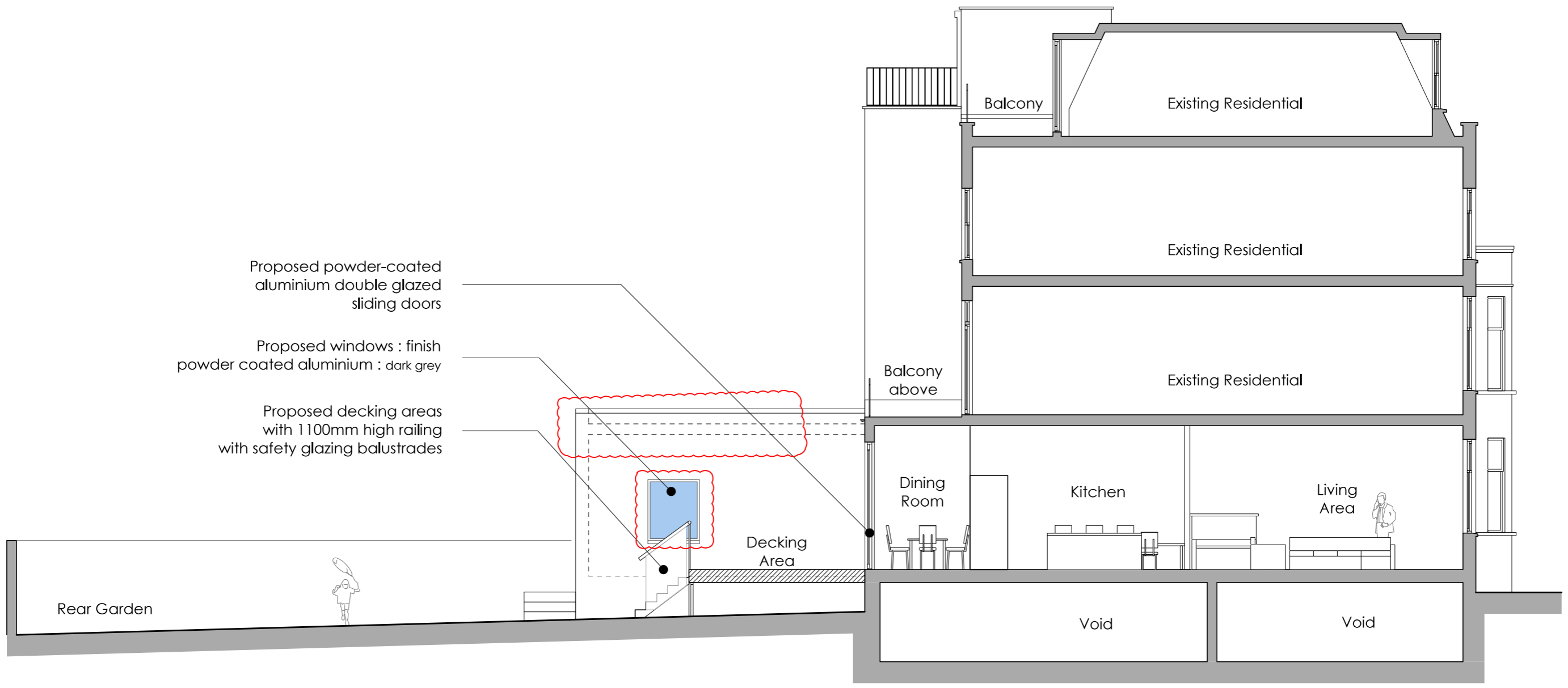
1 P-123 Proposed Side Elevation & Longitudinal Section scale 1:100 @ A3
