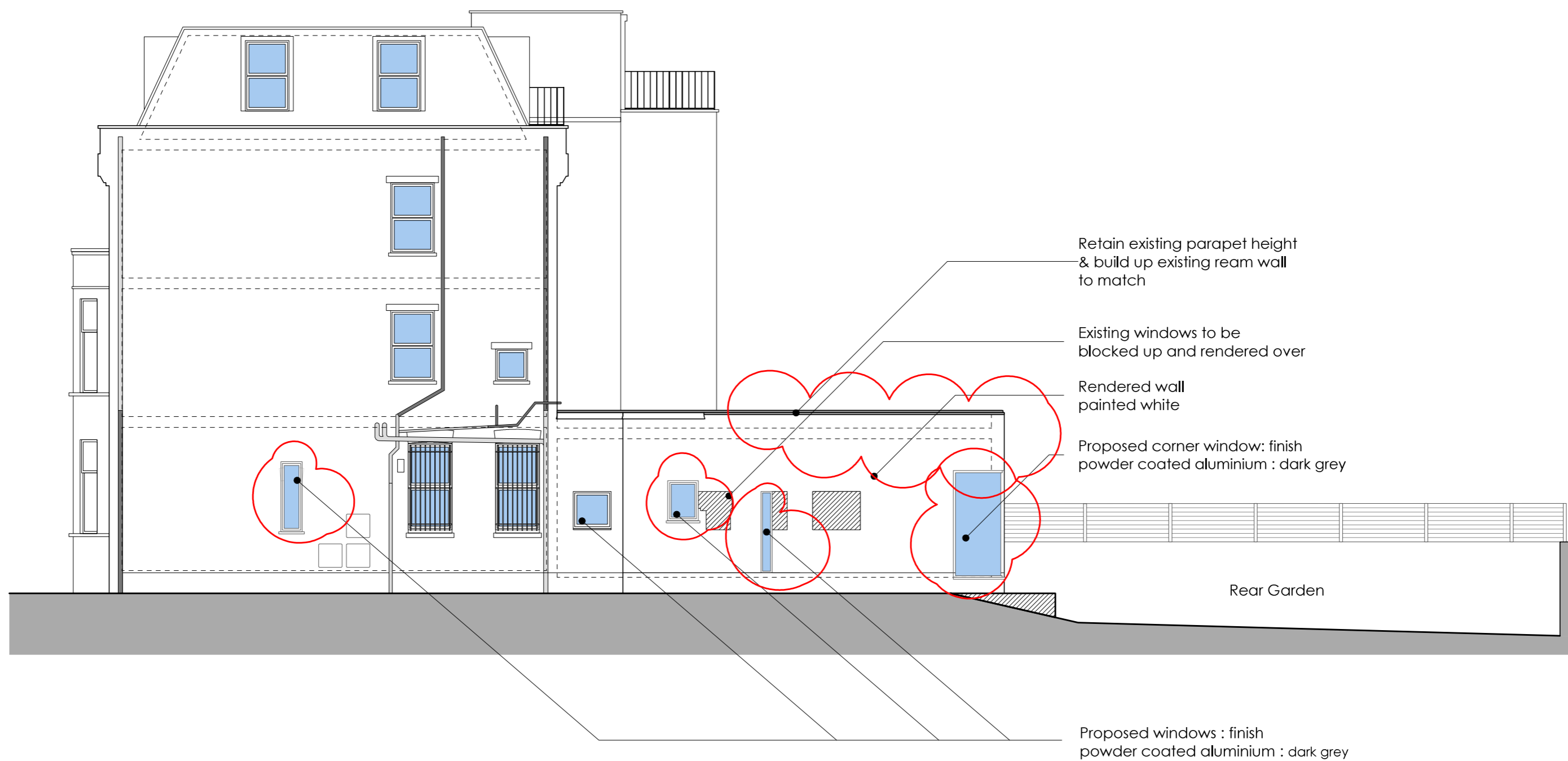
1 P-121 Proposed Side (West) Elevation scale 1:100 @ A3
