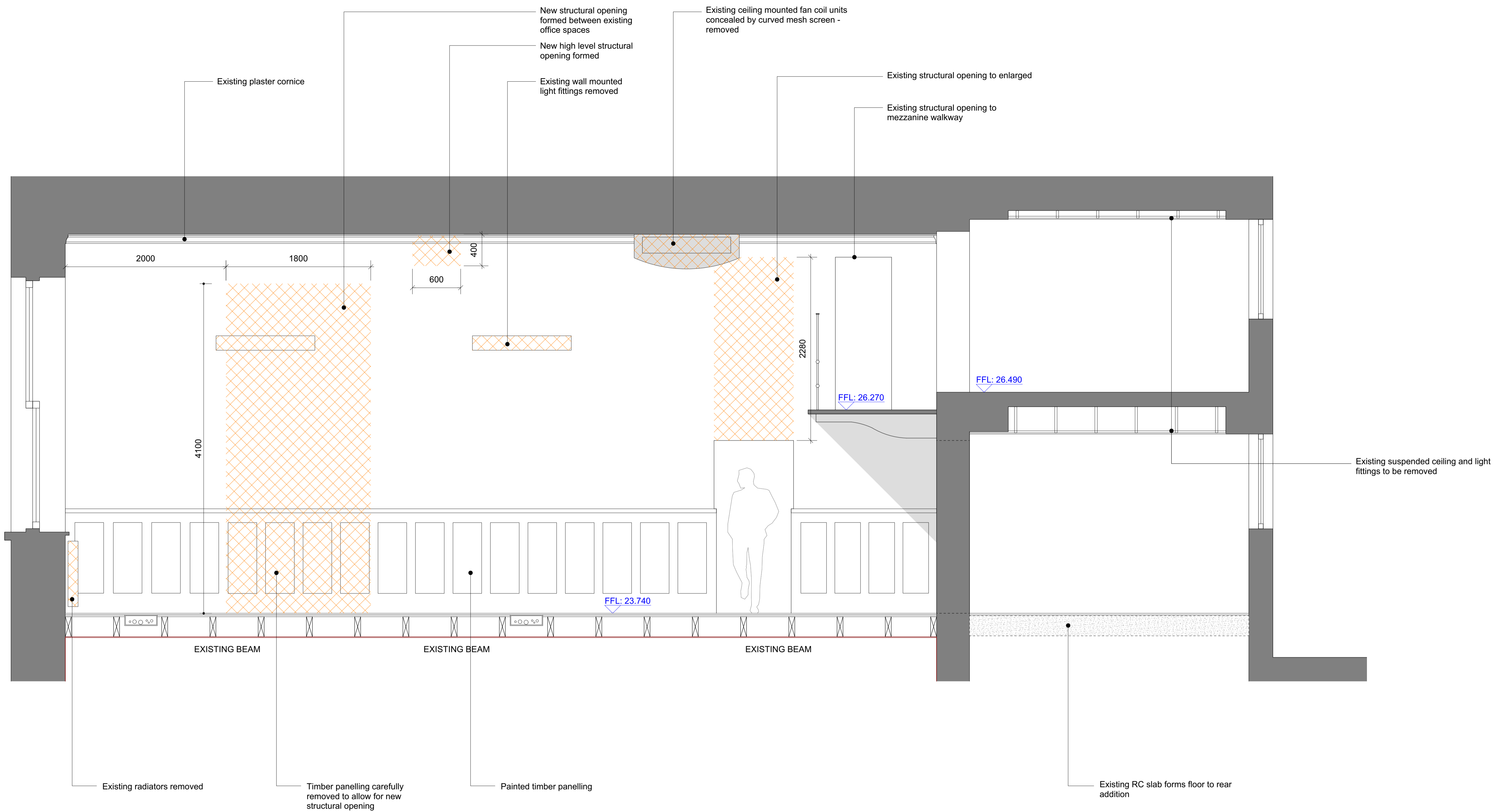
1 Existing Section AA (183 Eversholt St) Scale 1:50 @ A1 / 1:100 @ A3
