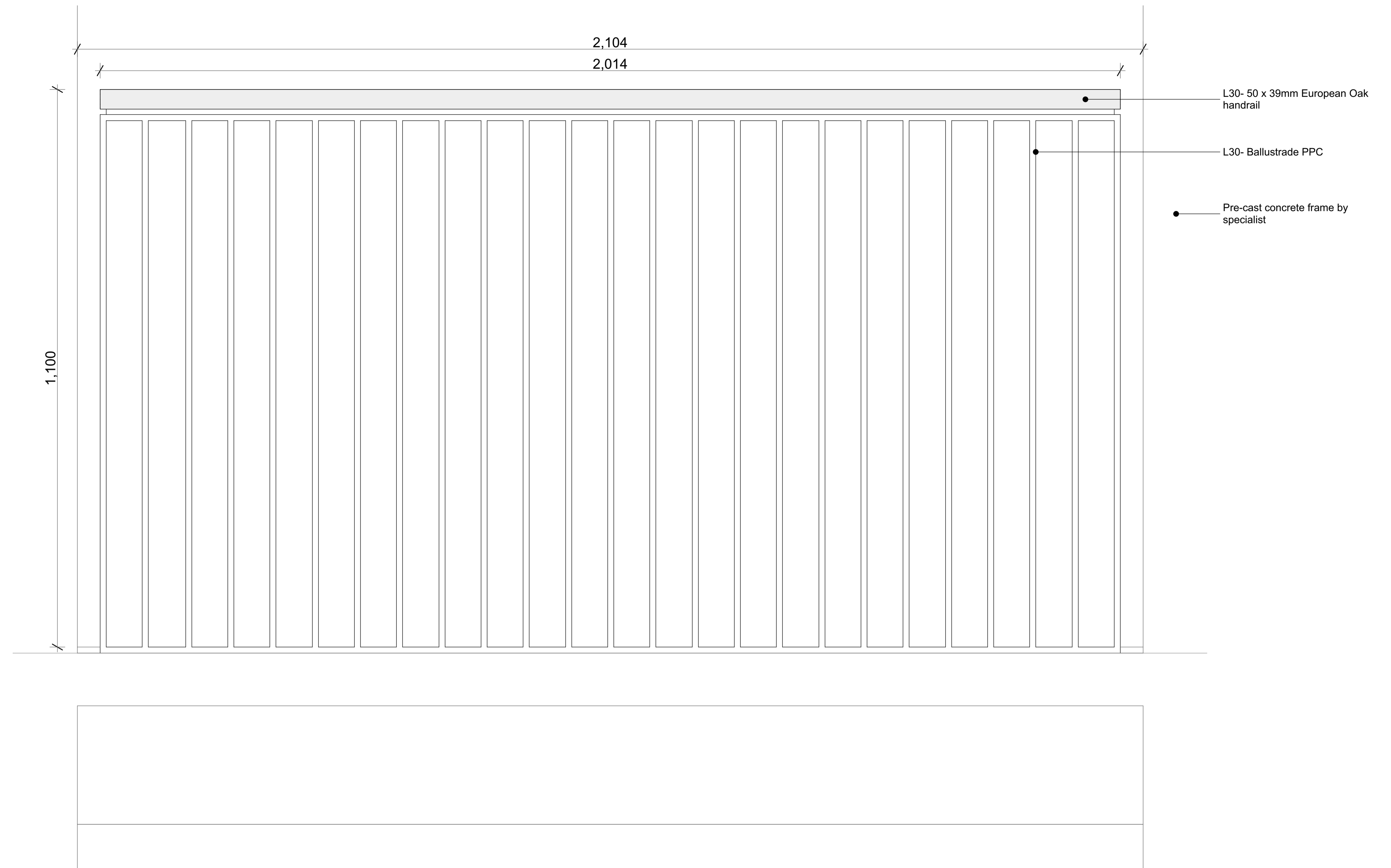
Z3_760_01 Elevation (1) 1:5
