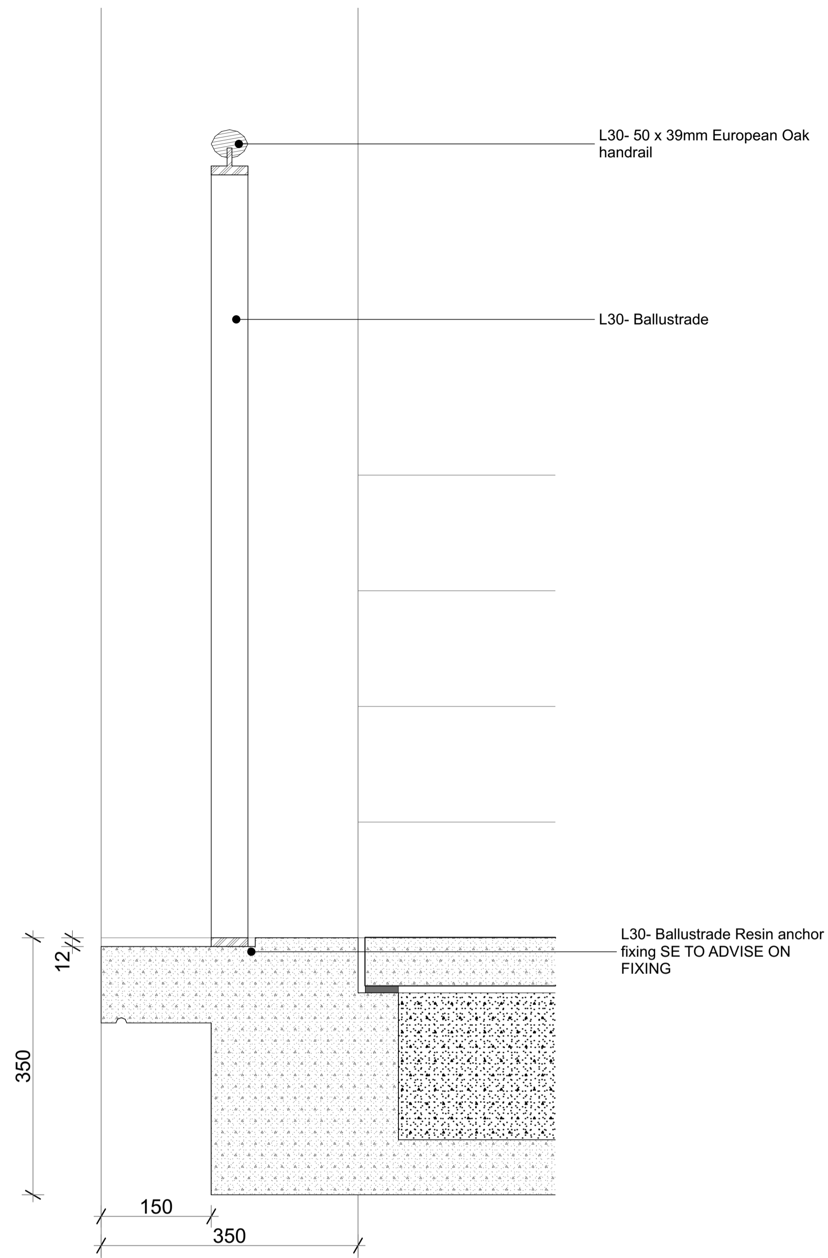
Z3_760_02 Section 1:5
