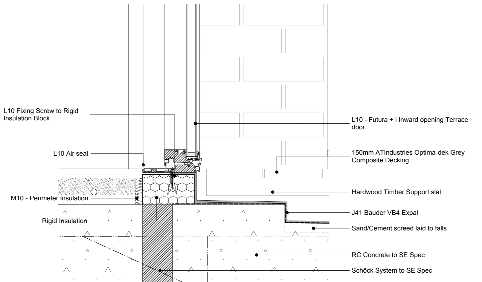
02 711 Typical Futura + inward opening terrace door balcony head/sill detail
