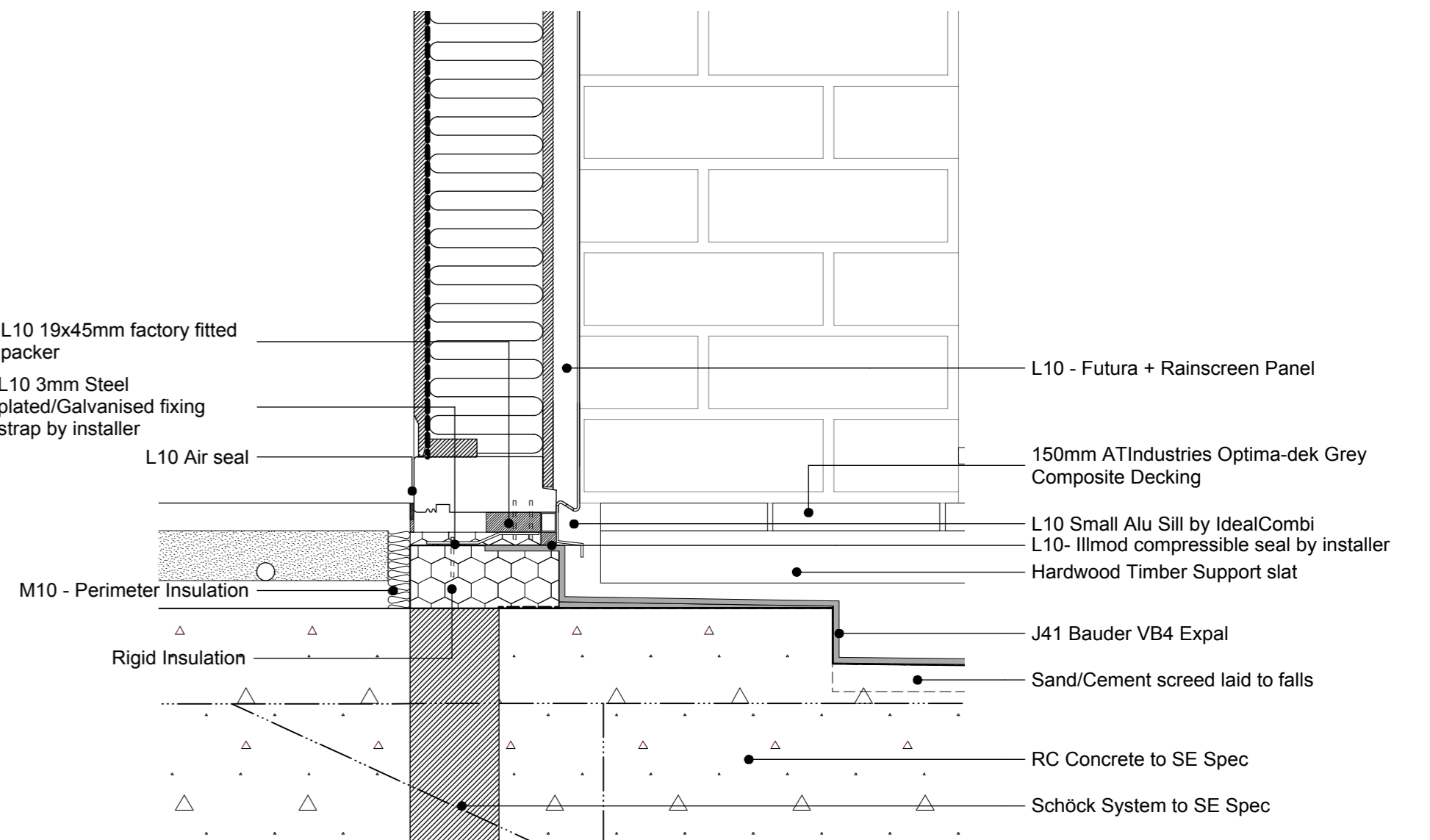
03 711 Typical Futura + rainscreen panel head/sill detail
