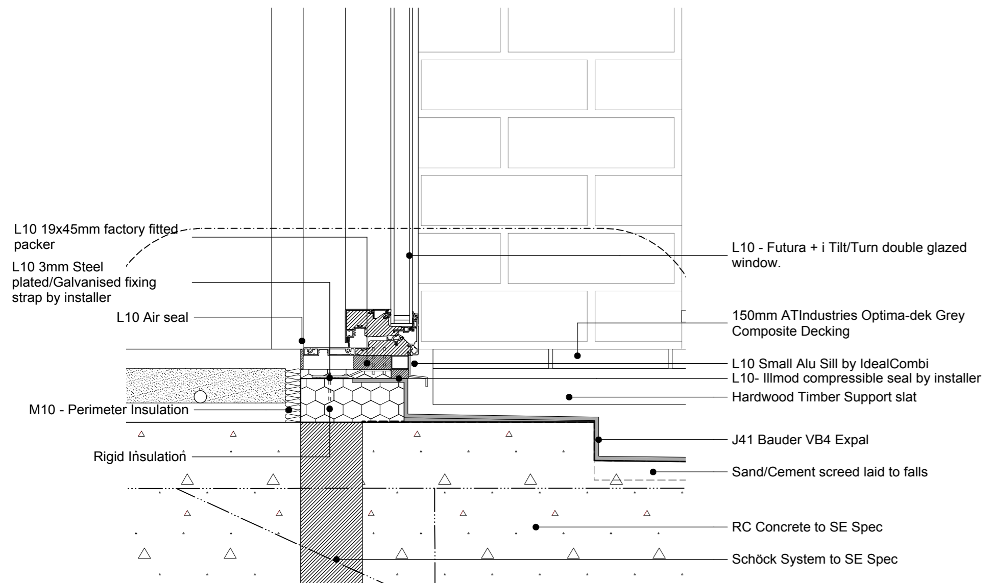
01 711 Typical Futura + balcony head/sill detail
