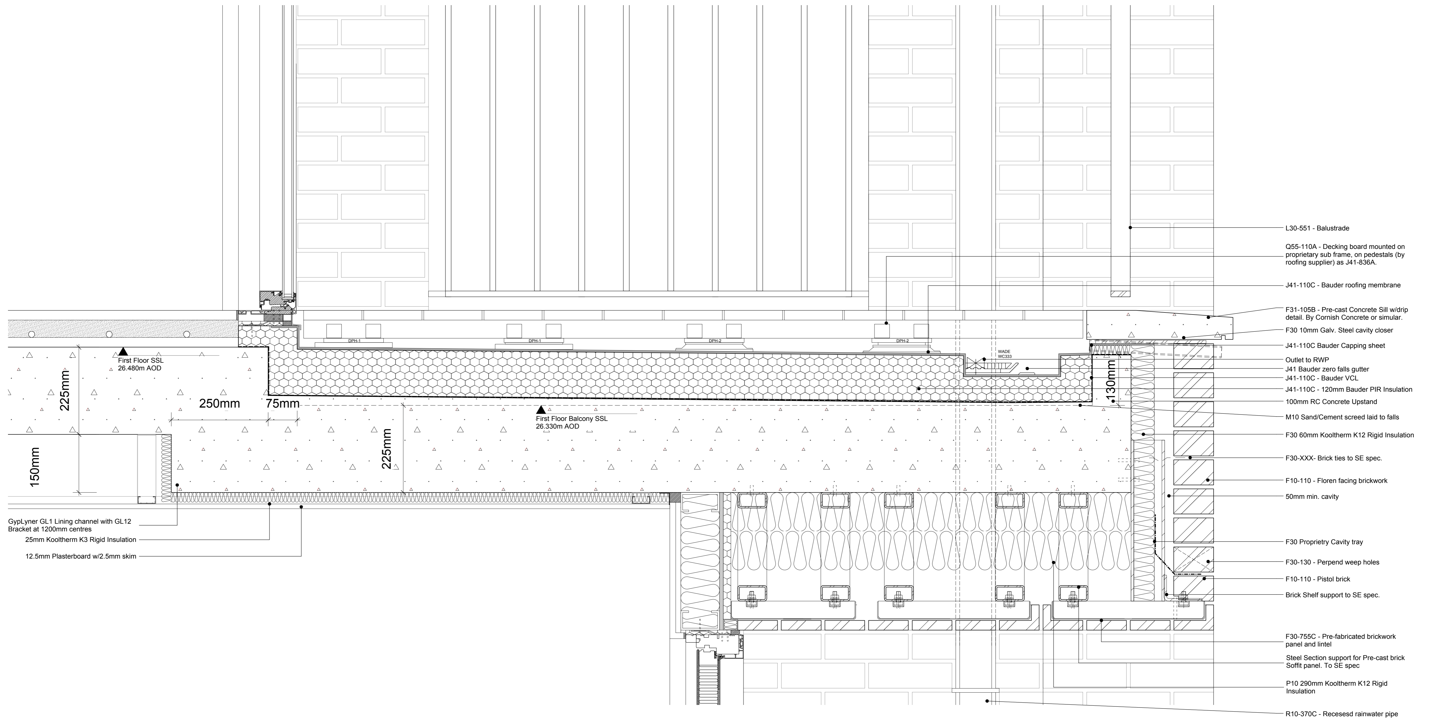
01 Devonshire Typical 1st floor balcony detail 611
