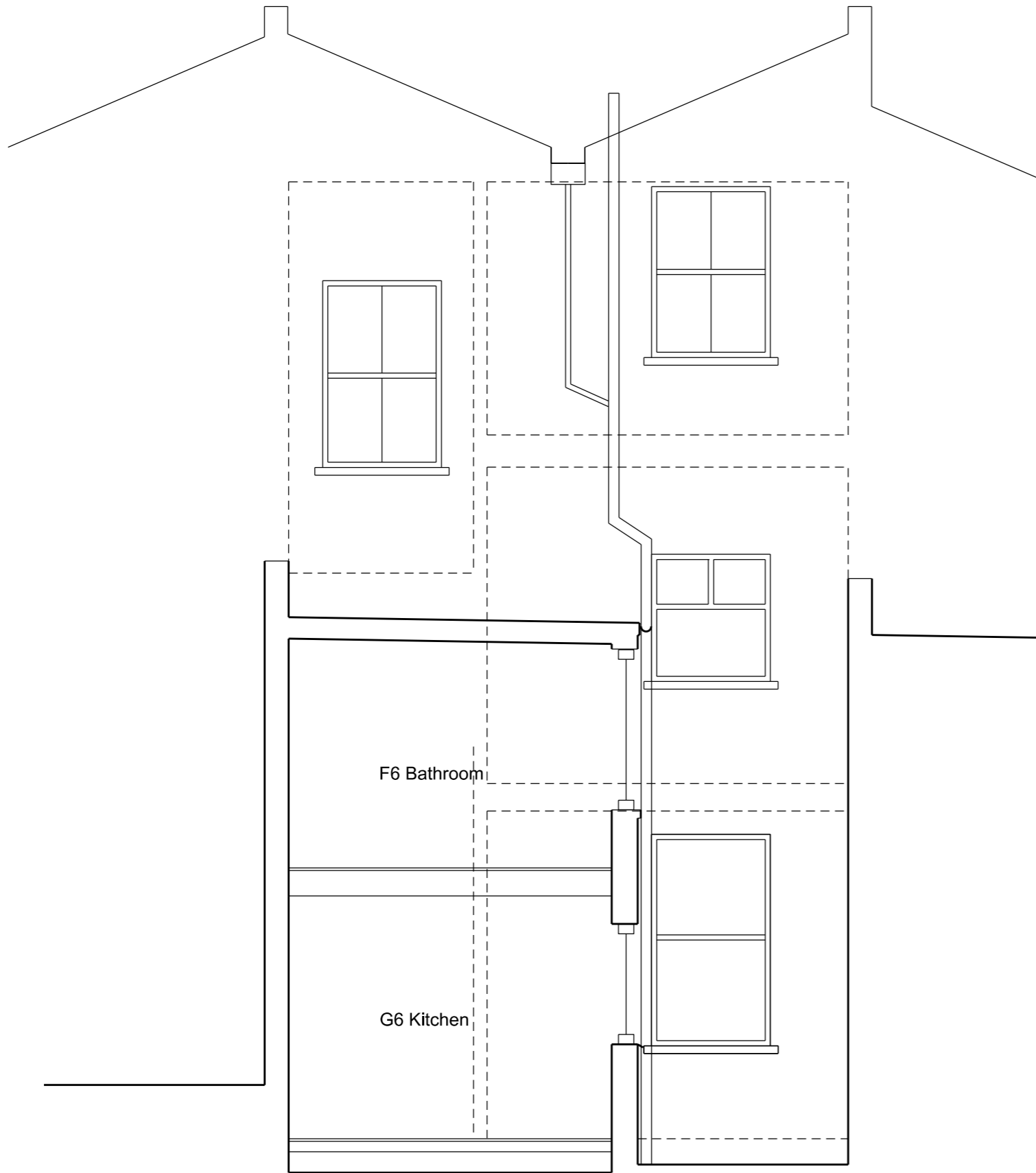
CROSS SECTION AS EXISTING 93 MESSINA AVENUE WEST HAMPSTEAD NW6 4LG
