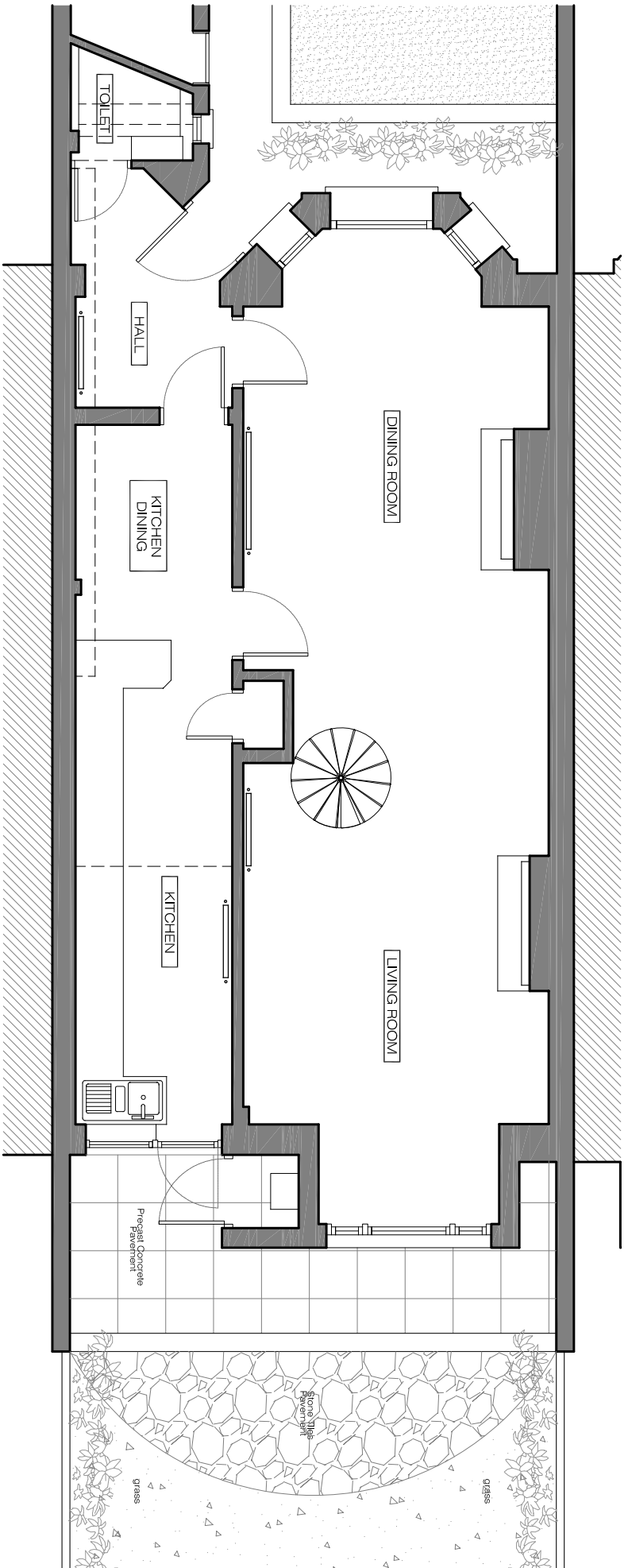
EXISTING LOWER GROUND FLOOR PLAN SCALE 1:50@A3 EX-01
