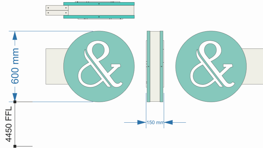
W&G-ES1.10-A Ø600mm Projecting Sign
