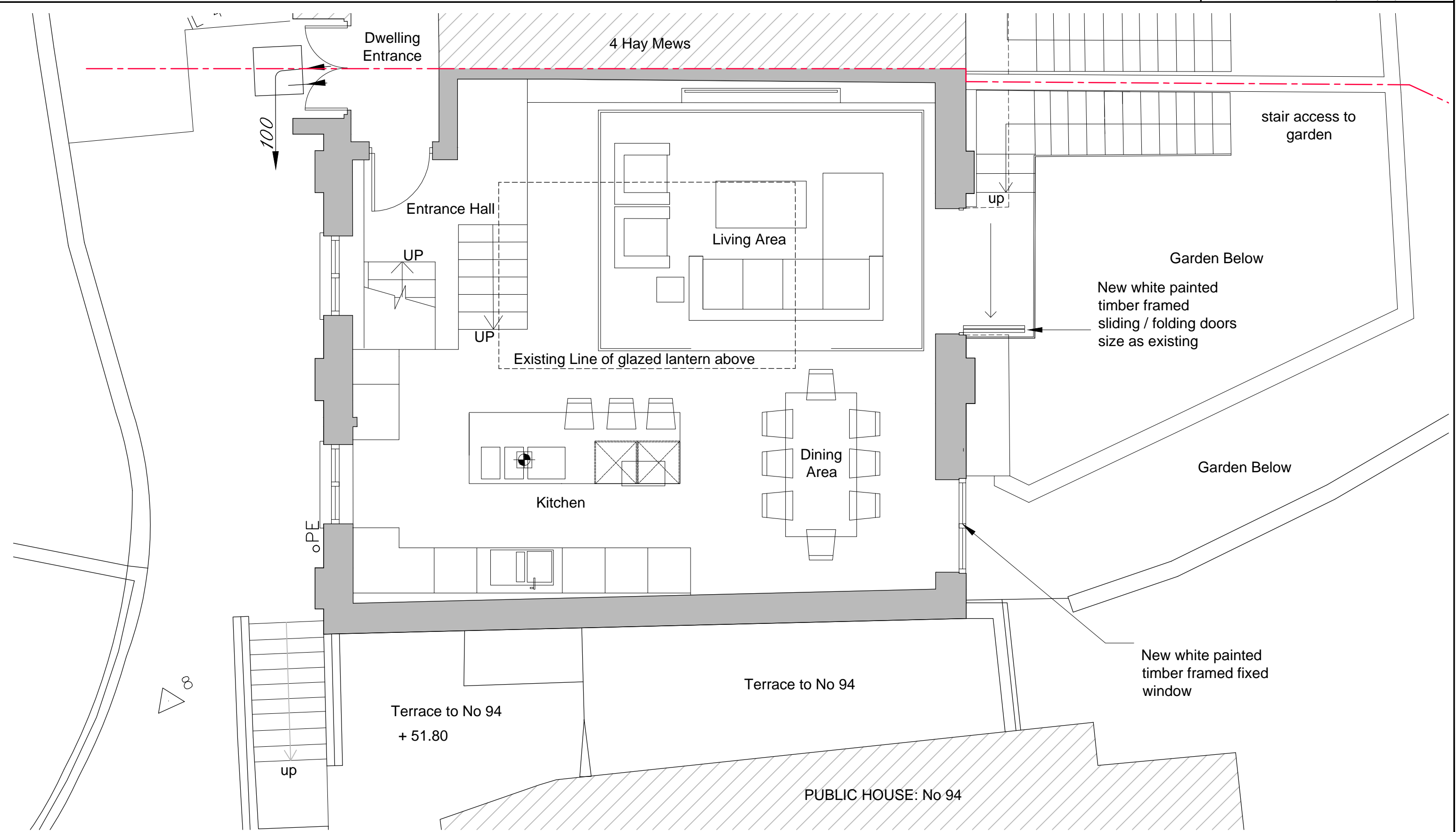
Proposed Upper Ground Floor Plan: 1:50 @ A3
