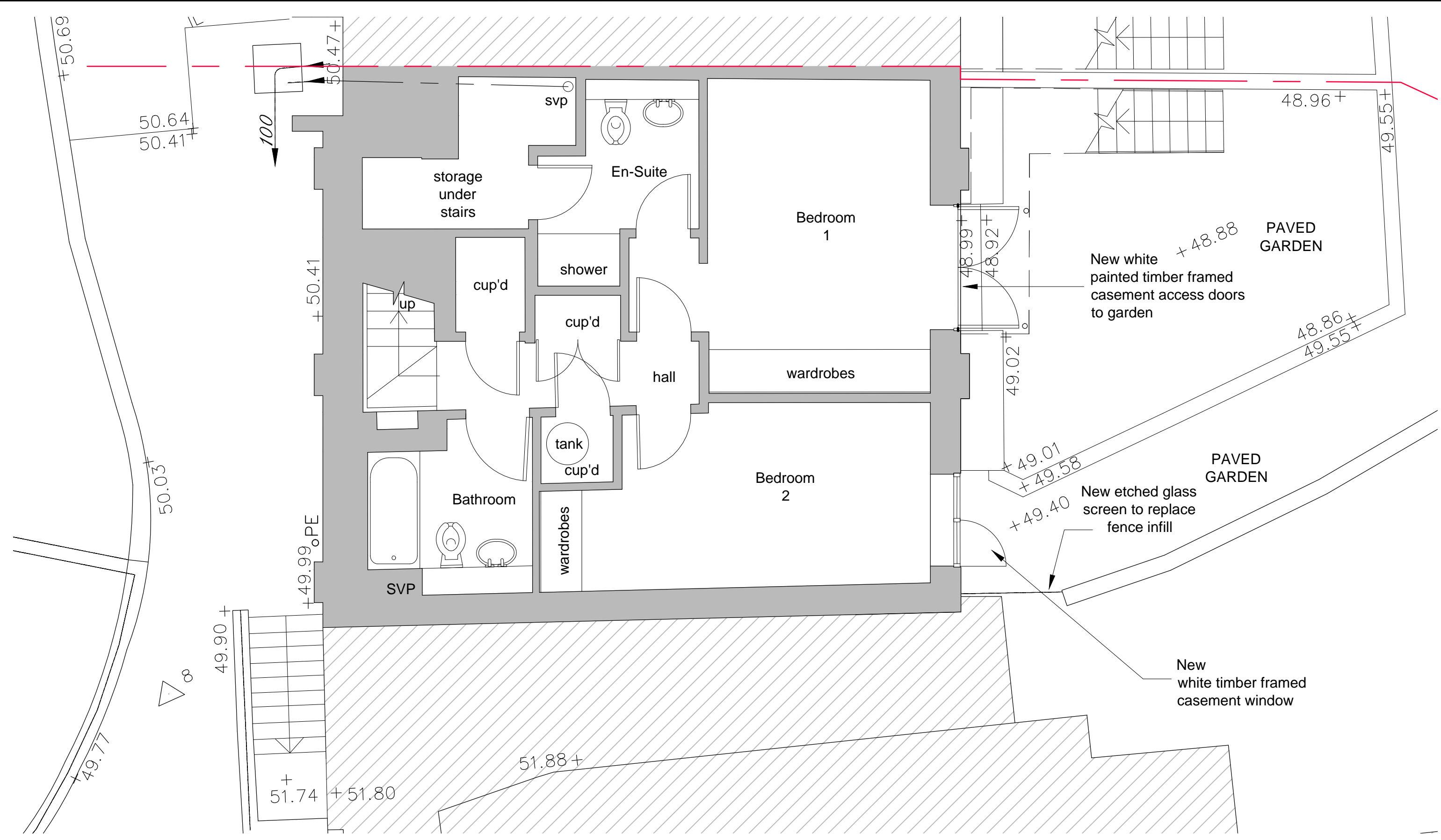
Proposed Lower ground Floor Plan: 1:50 @ A3
