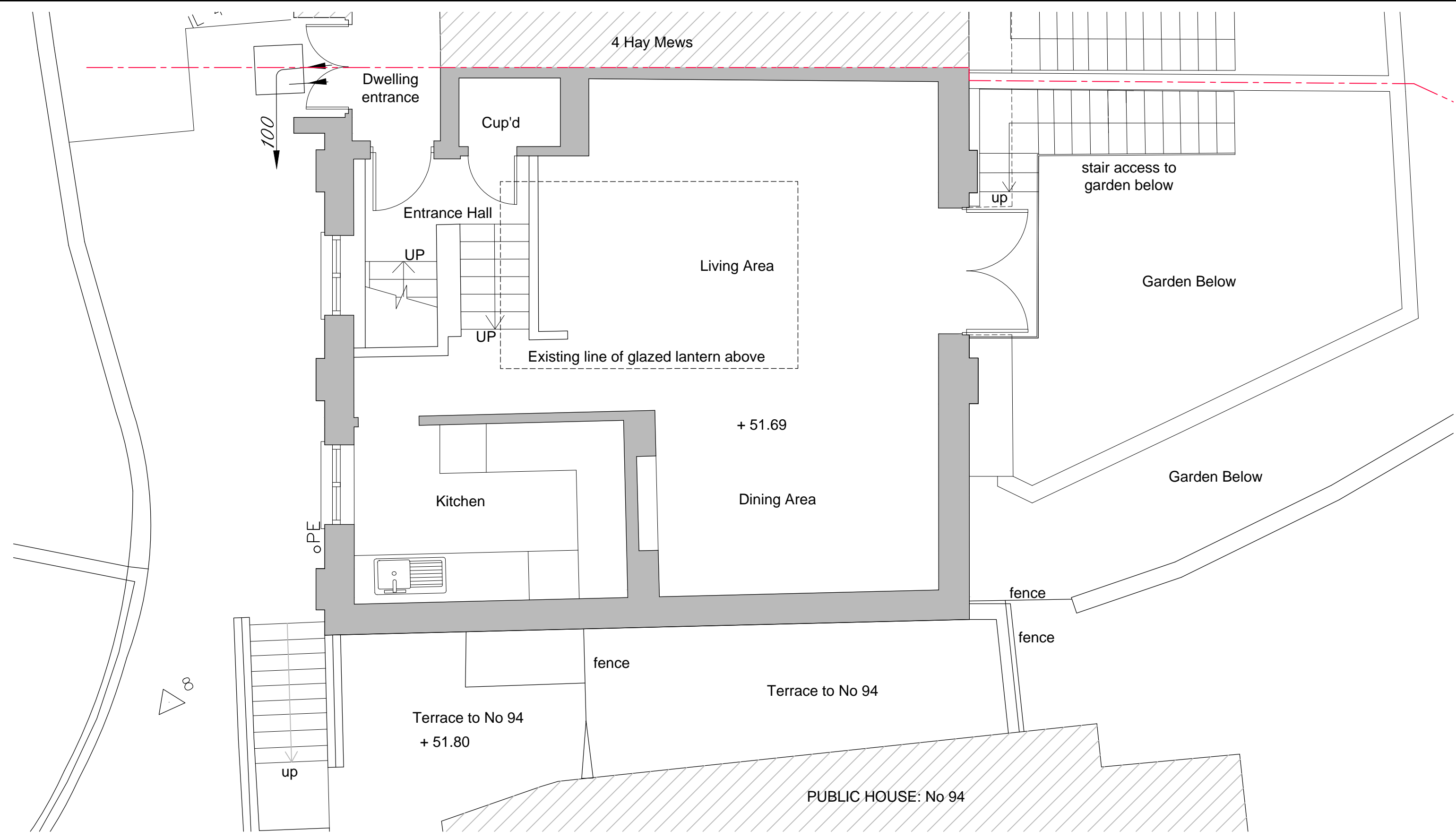
Existing Upper Ground Floor Plan: 1:50 @ A3
