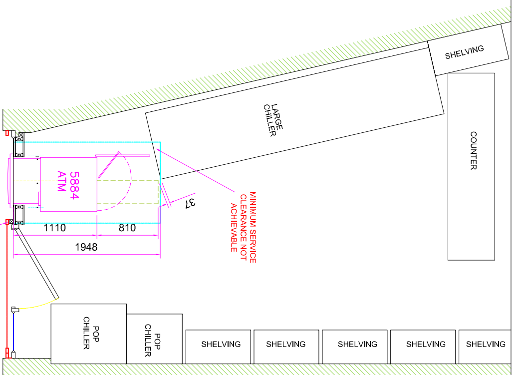
PROPOSED (PART) PLAN
