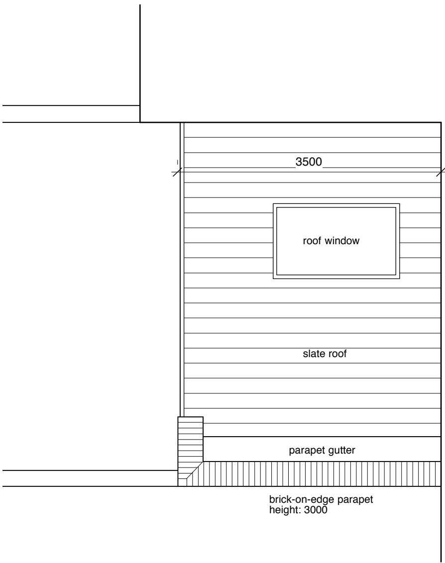
ROOF PLAN TO EXTENSION
