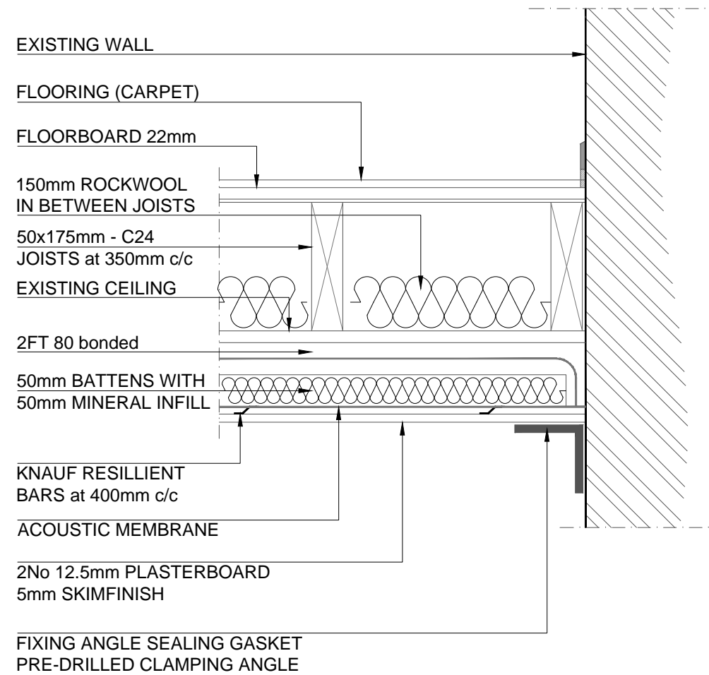
DETAIL 2 acoustic ceiling detail of separating the floors
