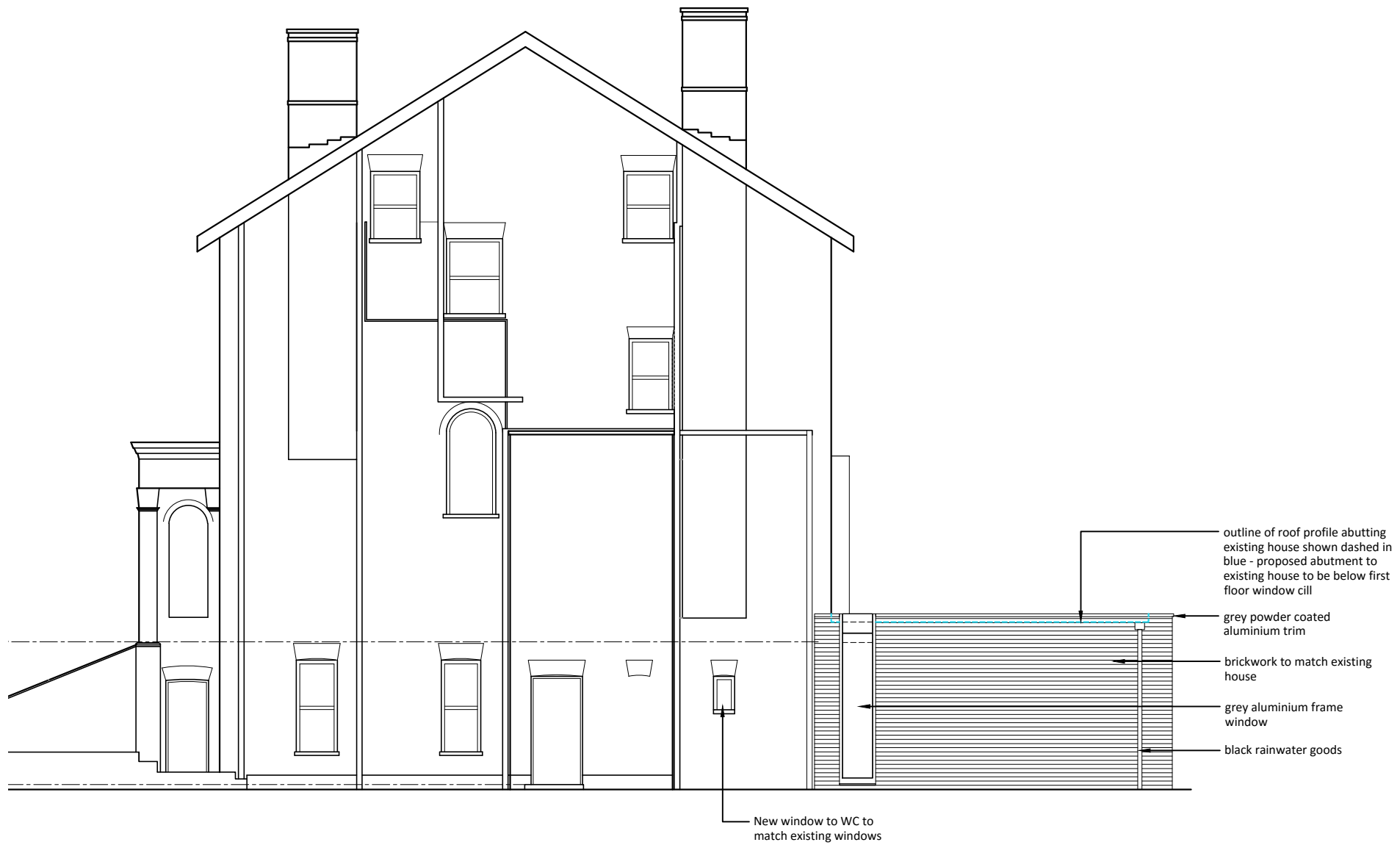
SIDE ELEVATION
