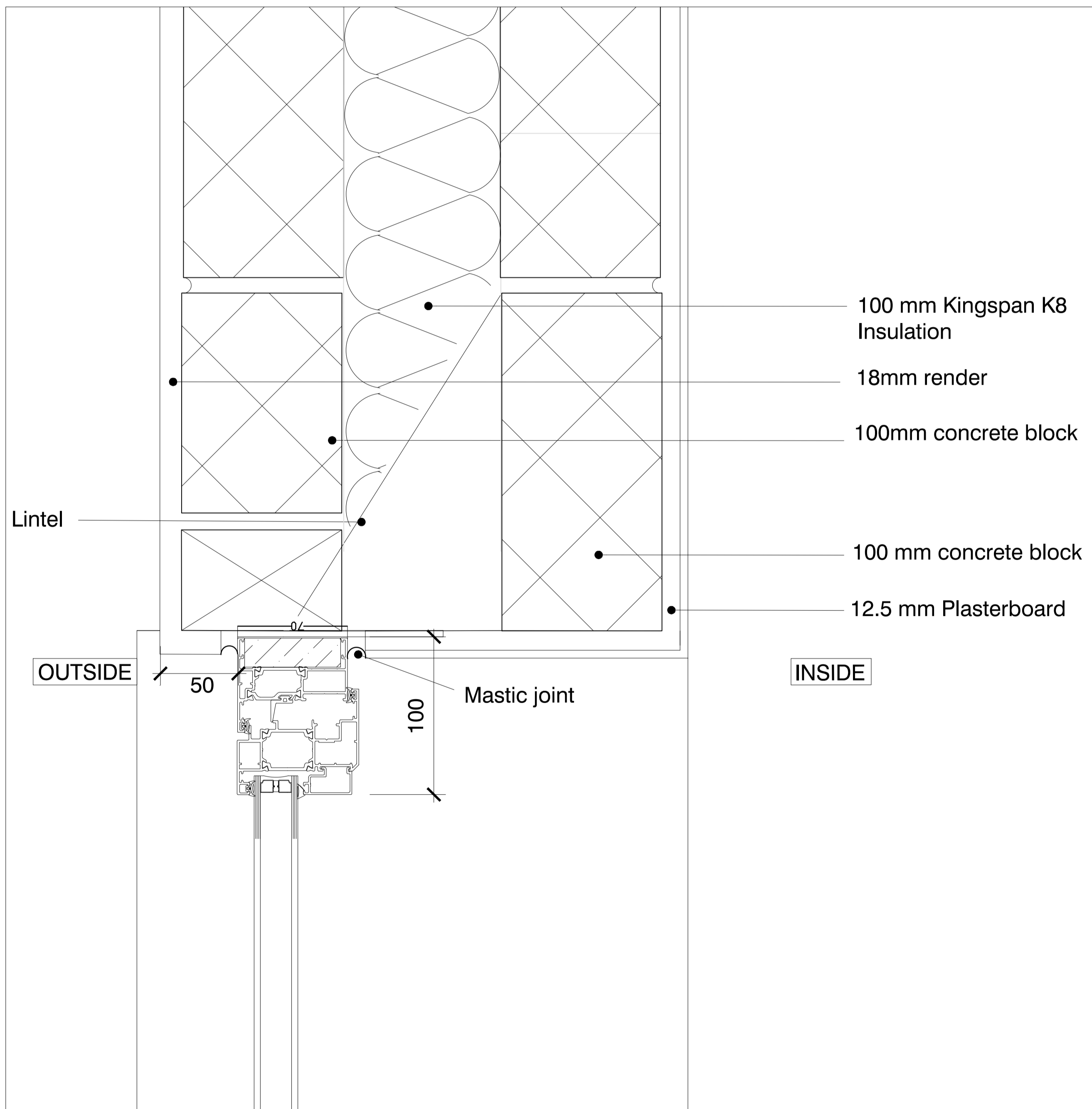
A(21) 02 EXTERNAL WALL STANDARD WINDOW DETAIL IN SECTION 1 1:5
