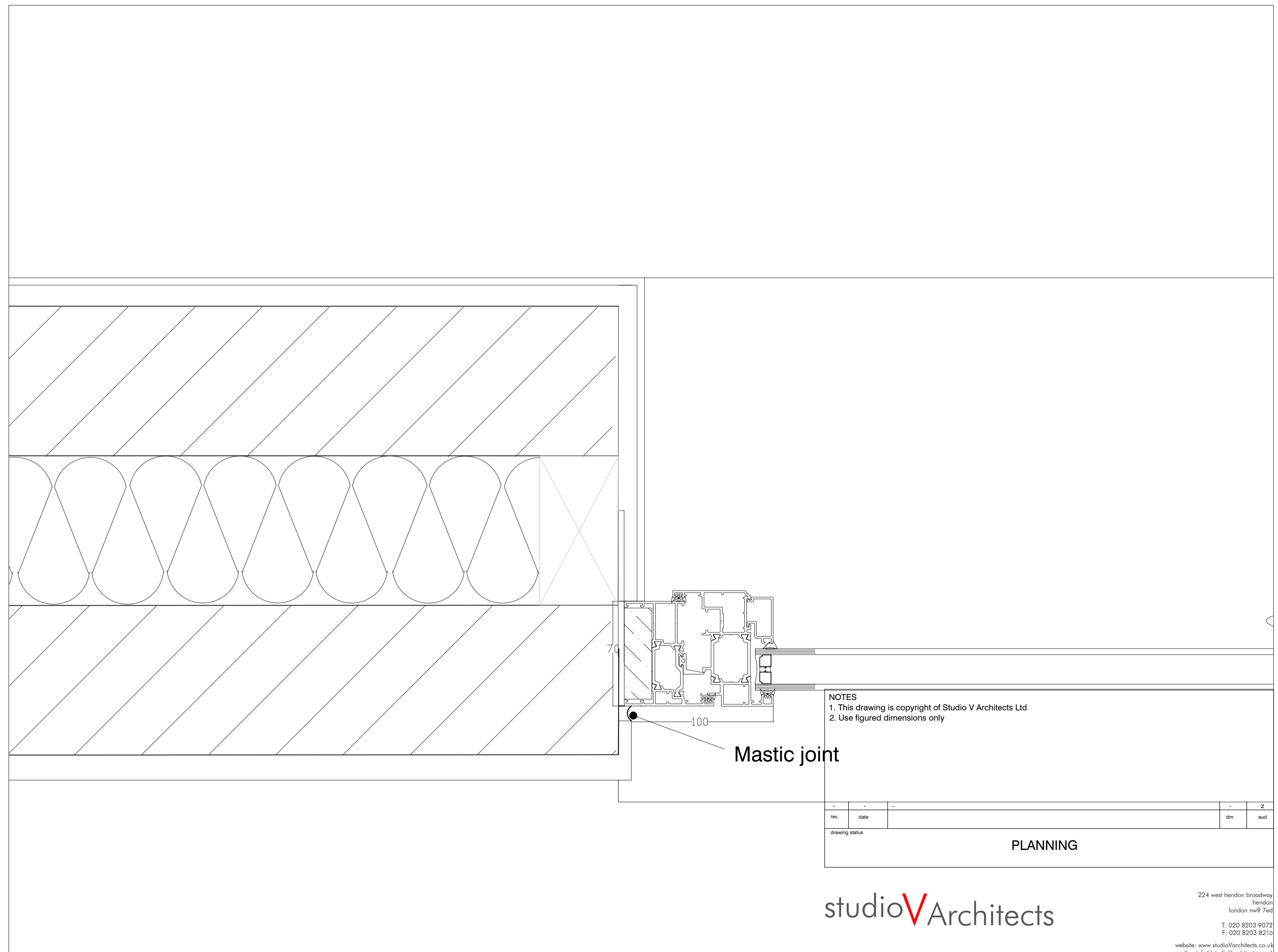
A(21) 02 EXTERNAL WALL WINDOW DETAIL IN PLAN 3 1:5
