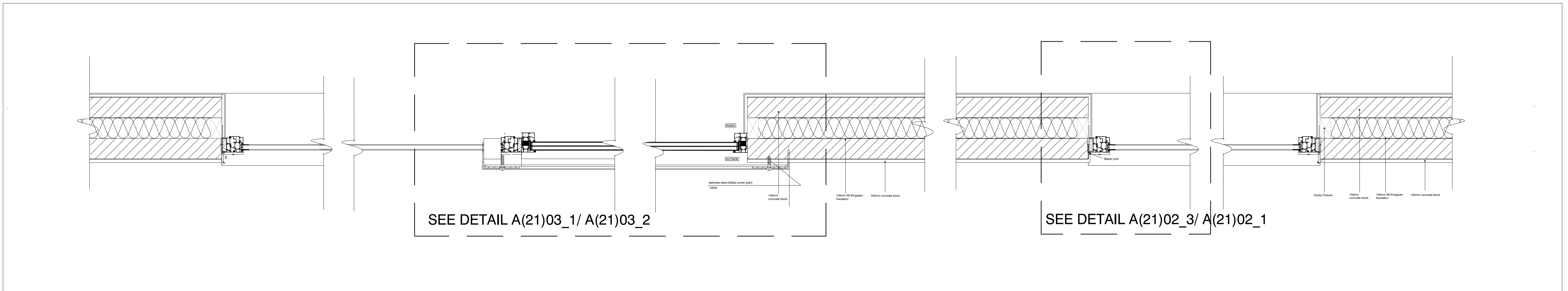
A(21) 02 EXTERNAL WALL STANDARD WINDOW/ DOOR DETAIL IN PLAN 2 1:10
