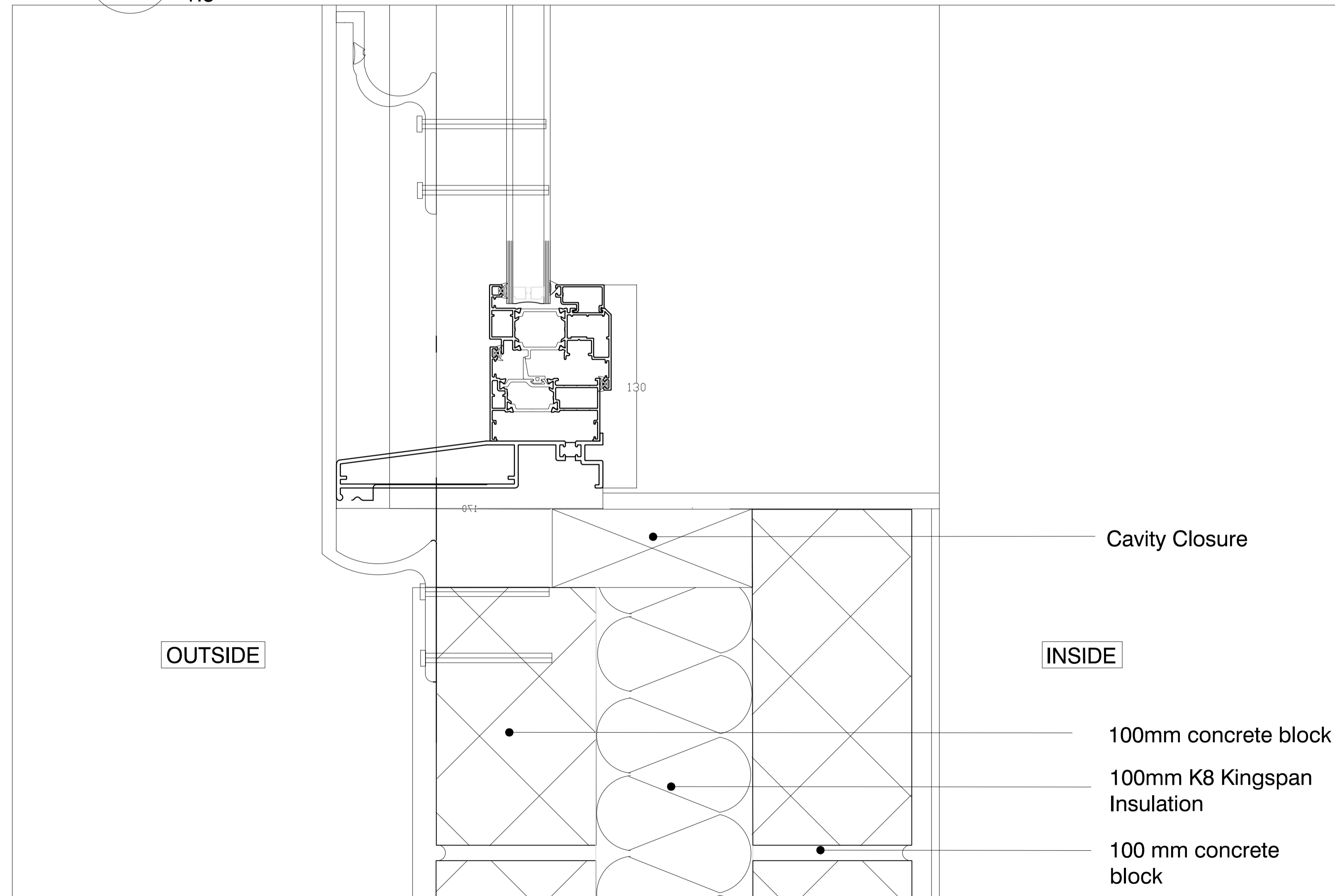
A(21) 03 EXTERNAL WALL JULIET WINDOW DETAIL
