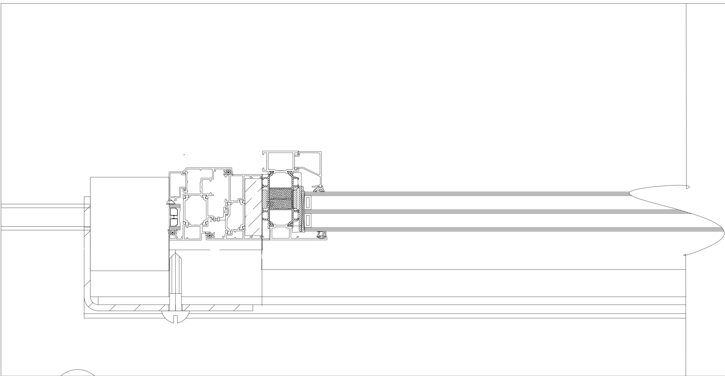
A(21) 03 EXTERNAL WALL JULIET BALCONY DETAIL
