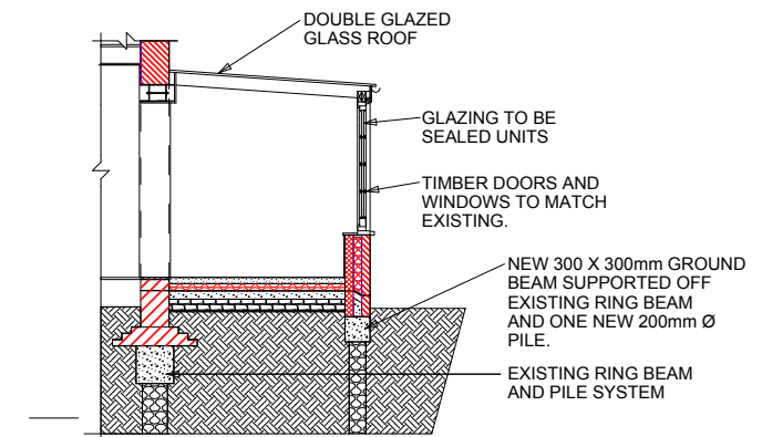
CROSS SECTION
