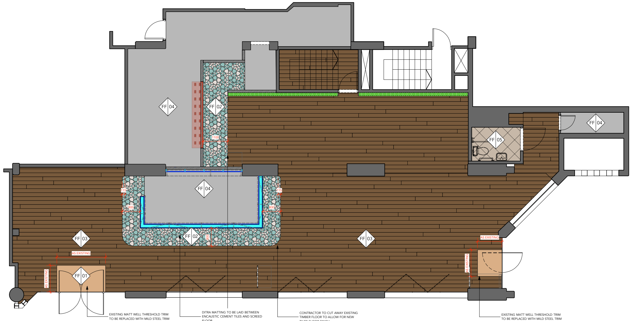
1 FLOOR FINISHES PLAN (GF) 1:50 @ A1 1:100 @ A3
