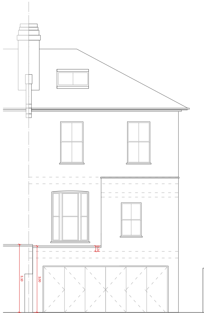
REAR ELEVATION E: 1/100
