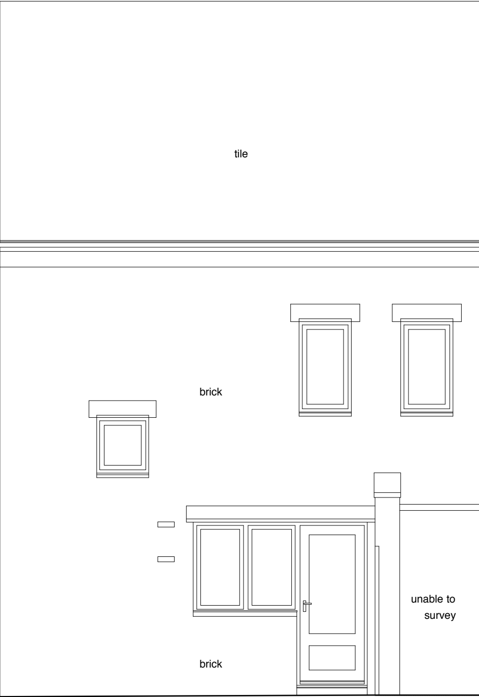
REAR ELEVATION
